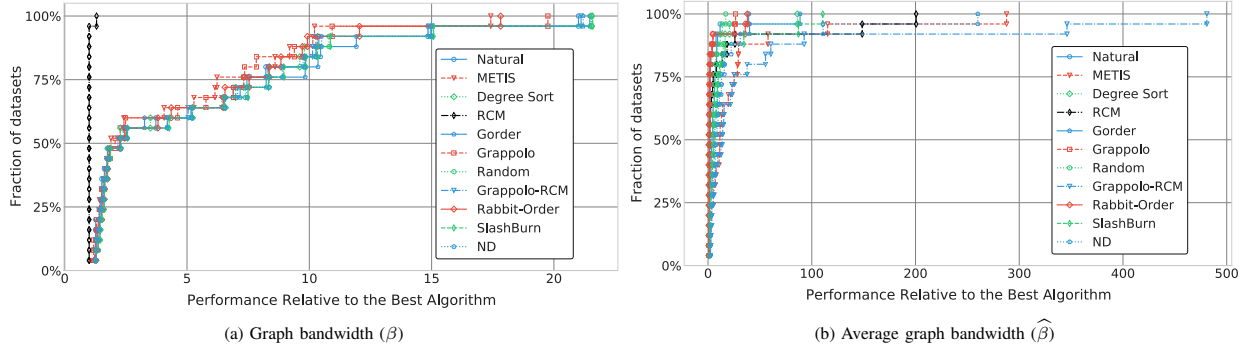
Fig. 6: Profile of relative performance of graph bandwidth (left) and average graph bandwidth (right). The Y-axis represents the fraction of problems with a total of 25 inputs. The X-axis represents the factor by which a given scheme fares relative to the best performing scheme over that fraction of inputs.
