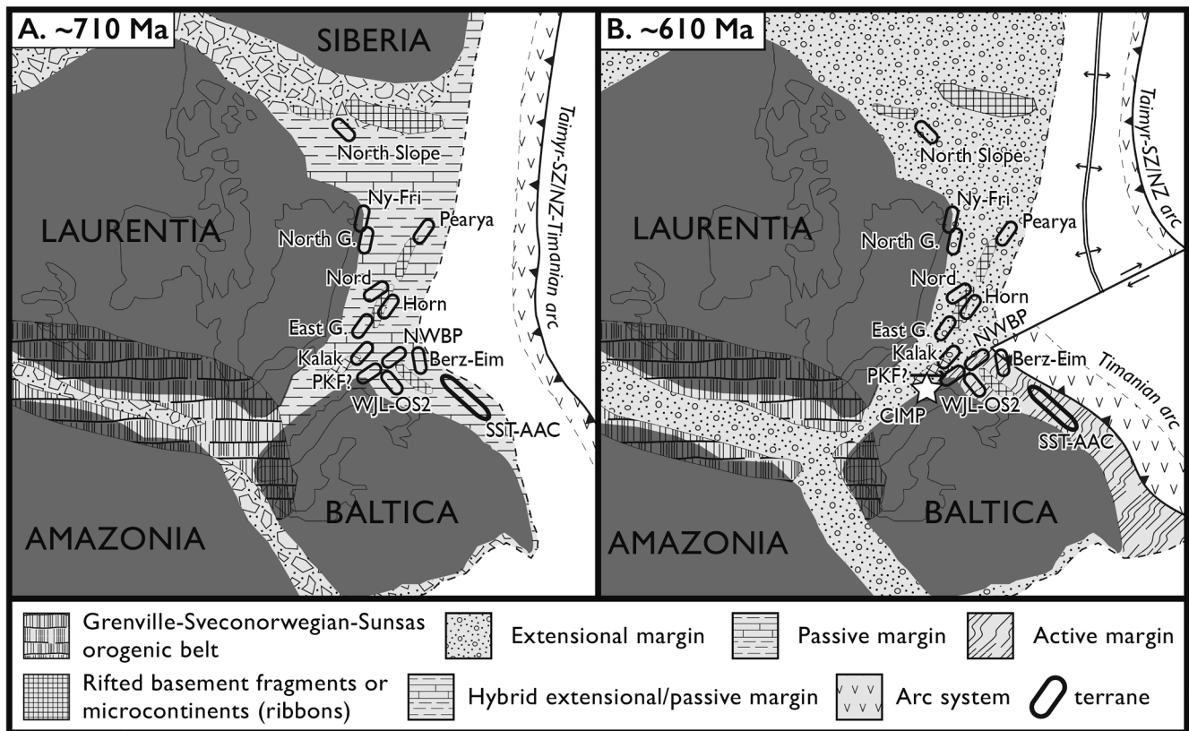
Fig. 18. Schematic Neoproterozoic paleogeographic reconstructions of the North Atlantic-Arctic Caledonides modified after Malone et al. (2014) and Bazarnik et al. (2019) . See text for discussion. North G.–North Greenland; Ny-Fri–Ny Friesland terrane, Northeast Basement Province of Svalbard; Nord–Nordaustlandet terrane, Northeastern Basement Province of Svalbard; East G.–East Greenland; Kalak–Kalak Nappe Complex of Norway; NWBP–Northwest Basement Province of Svalbard; Berz-Eim–Berzeliuseggene-Eimfjellet terrane, Southwestern Basement Province of Svalbard; WJL-OS2–Wedel Jarlsberg-Oscar II terrane, Southwestern Basement Province of Svalbard; PKF?–Prins Karls Forland terrane of the Southwestern Basement Province (question marks denotes uncertainty in affinity to Laurentia or Baltica); CIMP–Central Iapetus magmatic province (centralized location denoted by white star); SST-AAC–southwestern subterrane of the Arctic Alaska–Chukotka microplate.
