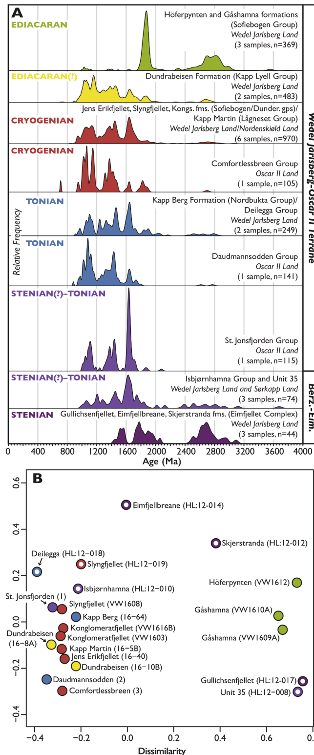
Fig. 15. A) Normalized probability density plots for detrital zircon U-Pb data from previously published samples in the Southwestern Basement Province and new samples presented herein from the Wedel Jarlsberg-Oscar II and Berzeliuseggene-Eimfjellet terranes. Prior to making this comparison plot, all data were filtered for >10% discordance, >5% reverse discordance, and >10% 2\sigma uncertainty in ^{206}\text{Pb}/^{238}\text{U} or ^{207}\text{Pb}/^{206}\text{Pb} ages. Errors were converted to 1\sigma and then the ^{206}\text{Pb}/^{238}\text{U} ratio was used to calculate an age for analyses younger than 1200 Ma and the ^{207}\text{Pb}/^{206}\text{Pb} result for analyses older than 1200 Ma. Published U-Pb data are from the following datasets: Deilegga Group (Sample HL:12-018; Ziemniak et al., 2019); Slyngfjellet Formation (Sample HL:12-019, Ziemniak et al., 2019); Isbjørnhamna Group (Samples HL:12-008, HL:12-010, and Sp21/08; Ziemniak et al., 2019); Eimfjellet Complex (Samples HL:12-012, HL:12-014, HL:12-017; Ziemniak et al., 2019); St. Jonsfjorden Group (Sample 1; Gasser and Andresen, 2013); Daudmannsodden Group (Sample 2; Gasser and Andresen, 2013); Comfortlessbreen Group (Sample 3; Gasser and Andresen, 2013). B) Multi-dimensional scaling (MDS) plot (Vermeesch, 2013) of the same data presented in A) except all samples are plotted individually. Samples with <50 individual zircon U-Pb analyses are shown as partially filled circles to highlight ambiguity for provenance comparison. Data were plotted using IsoplotR (Vermeesch, 2018). Kongs.-Konglomeratfjellet Formation; Dunder.-Dunderbukta Group; gps.-groups; fms.-formations.
