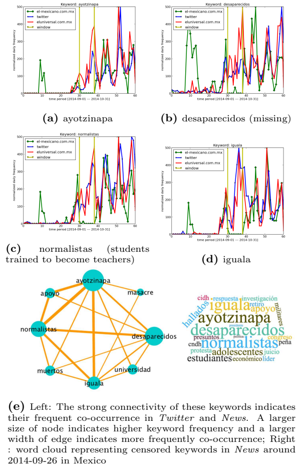
Figure 1: Example TSDF in News vs. TSDF in Twitter for a set of connected keywords. These keywords are relevant to the 43 missing students from Ayotzinapa Rural Teachers' College on Sep 26th, 2014 in Mexico. We can find consistent censorship pattern in El Mexicano Gran Diario Regional (el-mexicano.com.mx) shortly after the students are missing.
