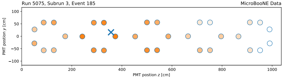
Figure 10. Example of a flash, consisting of multiple PMT signals combined. The orange colour scale is logarithmic and represents the intensity of the light, arriving in each PMT, integrated over 625 ns. The blue cross indicates the location of the centre of the flash. The 32 PMTs are organised in five rosettes, located behind the wires in the yz -plane.
