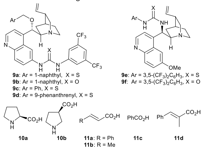
Figure 1. Structure of selected precatalyst modules and acids used in this study.
