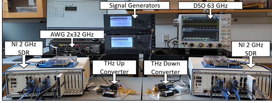
Figure 1. Ultrabroadband networking systems tested at Northeastern University.
