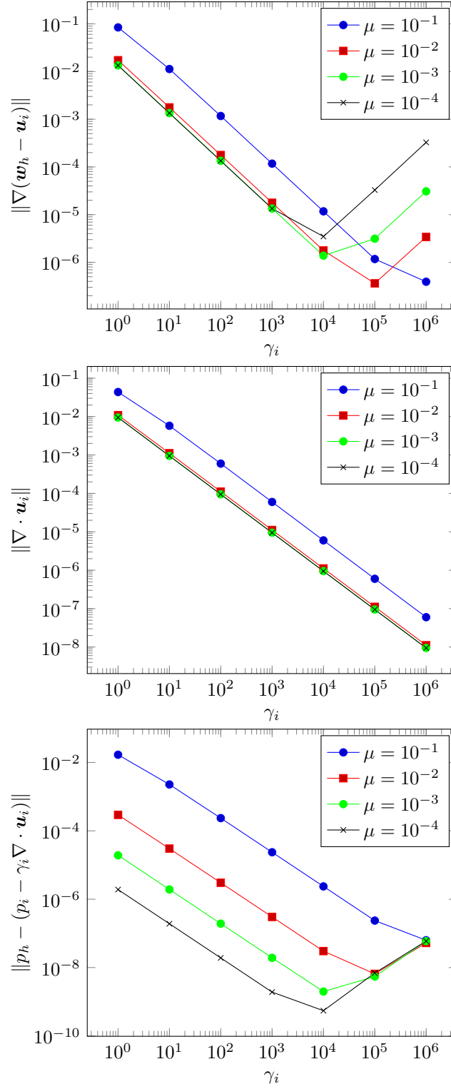
FIGURE 5. Numerical experiments using the \mathcal{P}_1 \times \mathcal{P}_0 pairs on Powell–Sabin splits with fixed h = 1/32 and varying viscosity \mu . Here, pr = p_i - \gamma_i \nabla \cdot u_i . The plot shows O(\gamma_i^{-1}) convergence for all three quantities. The increase in the first and third plots for large values of \gamma_i is due to round-off error.
