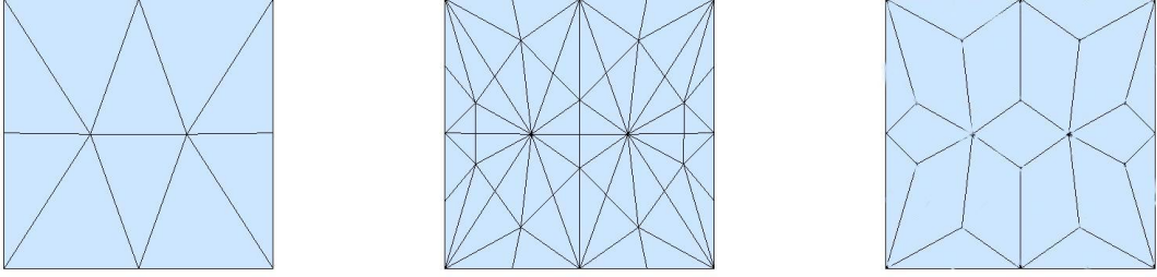
FIGURE 3. A triangulation \mathcal{T}_h of the unit square (left), its Powell-Sabin refinement \mathcal{T}_h^{PS} (middle), and the mesh \mathcal{K}_h^{PS} (right).
