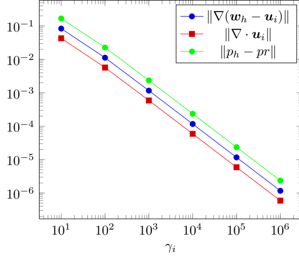
FIGURE 4. Numerical results on Powell-Sabin splits using the \mathcal{P}_1 \times \mathcal{P}_0 pairs for fixed h = 1/32 and viscosity \mu = 1 . Here, p_r = p_i - \gamma_i \nabla \cdot \mathbf{u}_i . The plot shows O(\gamma_i^{-1}) convergence for all three quantities.
