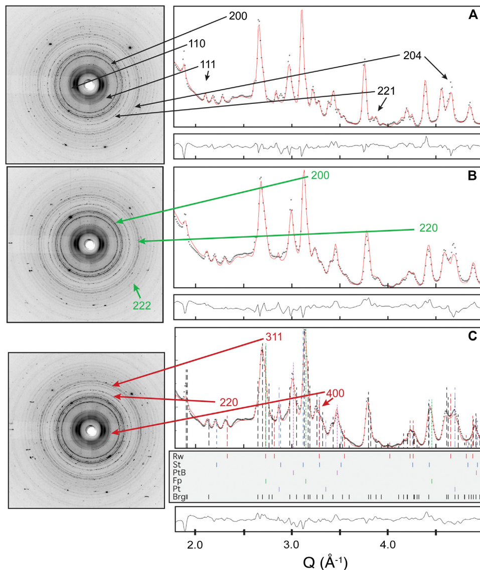
FIGURE 1 | Diffraction images (left) and Rietveld refinement fits for the average of all 5° spectra (right) from the software Materials Analysis Using Diffraction for (A) image 139 taken after raising the temperature of the converted aggregate to 1,000 K but before additional compression, (B) image 160 showing the partially compressed aggregate, and (C) image 172 taken at the final stage of compression. Colored, dashed vertical lines of arbitrary height indicate peak locations. Diffraction peaks used for reported Q(hkl) for bridgmanite, ferropericlase, and ringwoodite are labeled on plots (A), (B), and (C), respectively.
