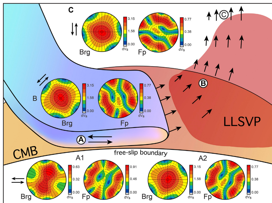
FIGURE 13 | Schematic diagram of shear wave splitting associated with a subducting slab in the D'' region. The slab is shown subducting along the core-mantle boundary (CMB). Large arrows show mantle flow around the edge of a large low-shear-velocity province (LLSVP). The schematic shows three possible locations of seismic anisotropy indicated by circled, capital letters: (A) deformation within the slab; (B) mantle flow at an angle to the CMB; (C) regions of upwelling. Uncircled letters refer to these regions and are adjacent to plots of percent shear wave splitting ( \delta V_s ) made for a hypothetical mantle "rock" composed of 80% bridgmanite and 20% ferropericlase at 100% strain. Plots labeled Brg show a case where bridgmanite textures and ferropericlase is randomly oriented. Plots labeled Fp show a case where ferropericlase textures and bridgmanite is randomly oriented. Arrows adjacent to plots indicate the sense of shear. In order to represent possible P/T variation in a subducting slab, region (A) includes CMB conditions (A1, 136 GPa and 4000 K) and a possible pressure/temperature condition at the top of the D'' (A2, 126 GPa and 2,800 K/3,000 K). A pressure and temperature condition of 126 GPa and 2,800 K/3,000 K was used for shear-wave splitting plots (B) and (C) . The black lines in the stereo plots are the orientation of displacement for the fast shear velocity ( V_{S1} , see text).
