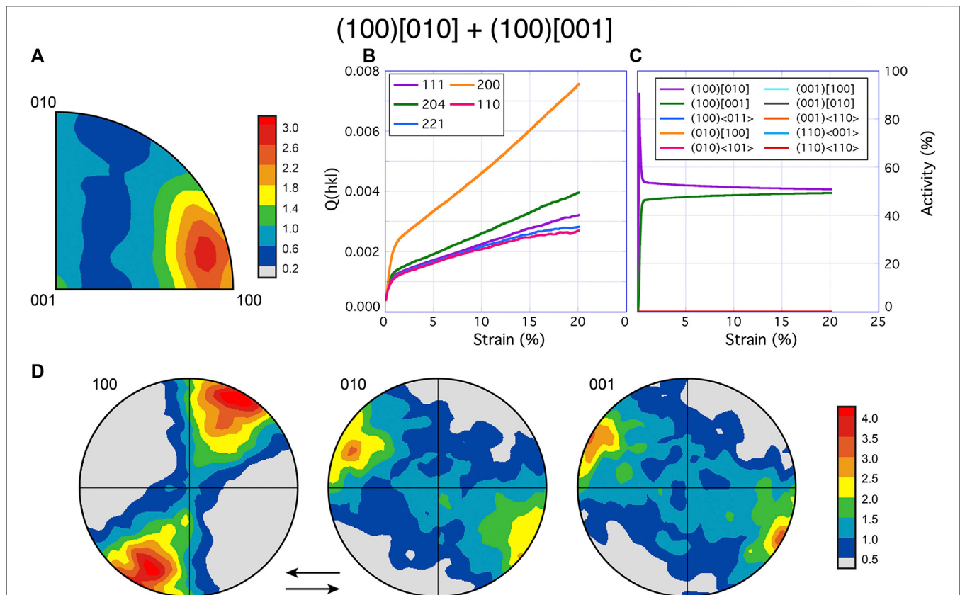
FIGURE 5 | Model results of bridgmanite for the slip system pair (100)[010] and (100)[001]. The results of elasto-viscoplastic self-consistent (EVPSC) modeling show (A) texture with color scales of the inverse pole figure (compression direction) given in multiples of random distribution. Q(hkl) and slip system activity are shown in plot (B) and (C), respectively. Pole figures (D) from VPSC models were simulated with the same critical resolved shear stress values as the EVPSC model. Shear orientation is top to the left, shown by the arrows. The activity of all but (100)[010] and (100)[001] is <1% at all conditions.
