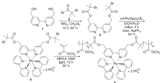
Scheme 1. Synthesis of 3 , 4 , and 5 .
