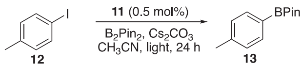
Scheme 4. Metal-free borylation of 12 carried out by polymer-supported 11 .
