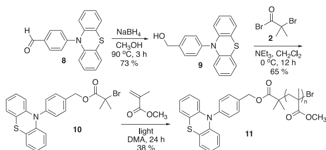
Scheme 3. Synthesis of 8 , 9 , 10 , and 11 .
