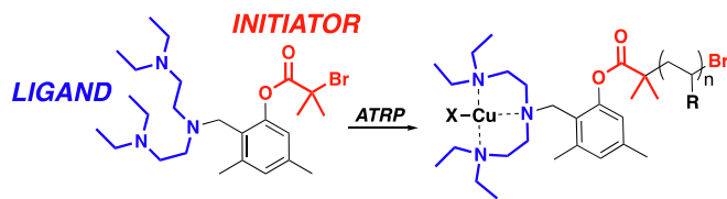
Fig. 1. ULIS-facilitated ATRP to prepare a metal-containing polymer from Ref. [26].
