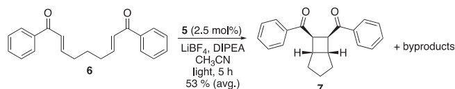
Scheme 2. [2+2] cycloaddition of 6 facilitated by polymer-supported 5 .
