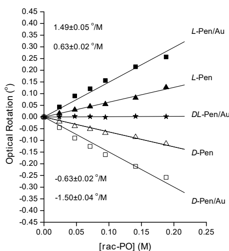
Figure 6. Optical rotation versus RS-PO concentration during addition to solutions containing Au-NPs coated with L-Pen (■), D-Pen (□) and DL-Pen (★). Addition of RS-PO to solutions containing enantiomerically pure D-Pen (Δ) and L-Pen (▲) indicates some interaction between PO and Pen. The concentration of Au was 0.24 M and the concentration of D-, L- and DL-Pen was 0.025 M.
