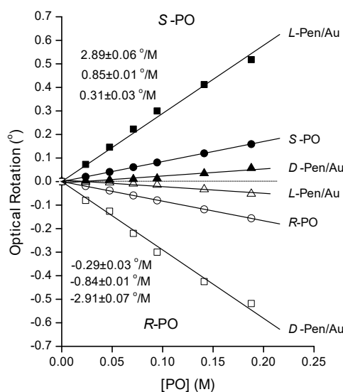
Figure 4. Optical rotation versus concentration of enantiomerically pure R- or S-PO in water and in solutions containing L- or D-Pen/Au-NPs. In aqueous solution, (● and ○), pure R- and S-PO rotate light with a specific rotation of \pm 0.85 \pm 0.01^\circ/\text{M} . In the presence of L- or D-Pen/Au-NPs, the optical rotation for S-PO changes from 2.9 to 0.3^\circ/\text{M} . The concentration of Au was 0.24 M and the concentration of Pen was 0.025 M.
