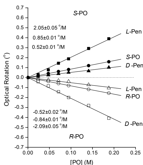
Figure 5. Optical rotation by enantiomerically pure R- and S-PO in water and in aqueous solutions of enantiomerically pure L- or D-Pen. In aqueous solution (● and ○), pure R- and S-PO rotate light with a specific rotation of \pm 0.85 \pm 0.01 °/M. In the presence of enantiomerically pure L- or D-Pen, the optical rotation of S-PO changes to 2.1 and 0.5 °/M, respectively. The optical rotations of R-PO are related to those of S-PO by diastereomerism. The concentration of D- and L-Pen was 0.025 M.
