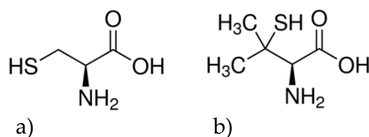
Figure 1. The molecular structures of (a) L-Cys and (b) L-Pen differ only in the addition of two methyl groups to the terminal carbon.
