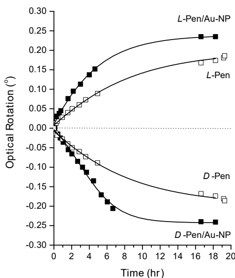
Figure 3. Optical rotation versus time by L- and D-Pen-coated Au-NPs and enantiomerically pure L- and D- Pen after exposure to a solution of 0.023 M RS-PO. The curves for D- and L-Pen are fits of a first-order exponential growth curve. The concentration of Au was 0.24 M and the concentration of Pen was 0.025 M.
