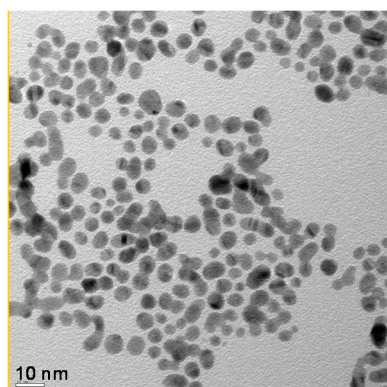
Figure 2. TEM image of Au-NPs. Nanoparticles are roughly spherical.
