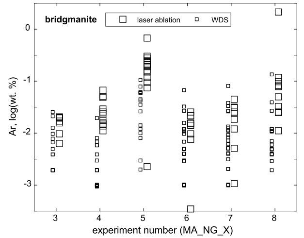
Fig. 4. Comparison of laser-ablation and WDS analyses of Ar concentrations in Brg from MA experiments. Both analytical techniques reveal highly heterogeneous Ar concentrations in all experiments that range from >0.1 to <0.01 wt.%.
