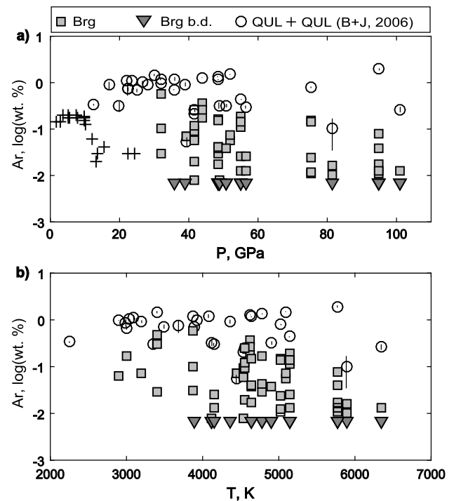
Fig. 6. Argon concentration measurements on QUL (circles) and Brg (squares) plotted as a function of a) pressure and b) temperature. QUL data points are the average of repeat measurements of individual experiments. Vertical lines associated QUL data points are one standard deviation of the mean. Brg data points are individual measurements of experiments and analyses yielding Ar concentrations below detection are plotted as down-pointing triangles. A subset of Ar analyses on Brg remains below detection, while QUL analyses extend above 1 wt.%, across the range of P - T conditions explored.
