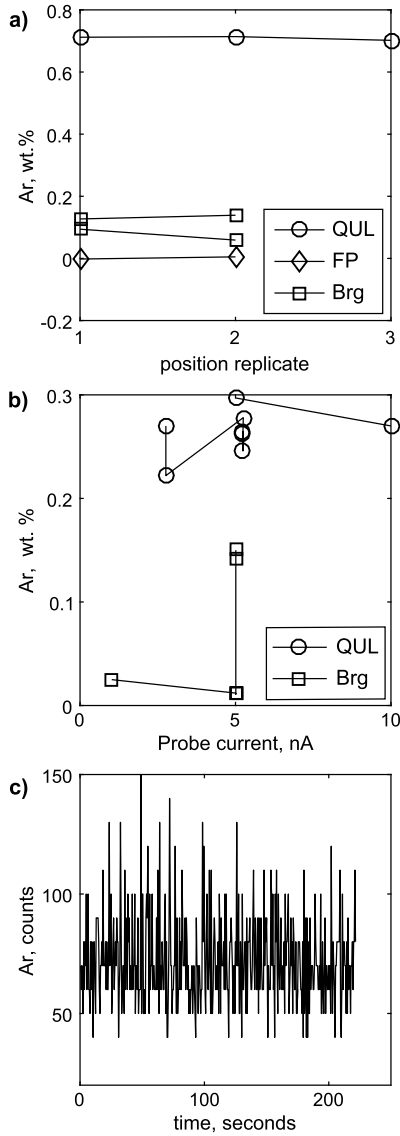
Fig. 3. Replicate Ar analyses of Brg, FP, and QUL to evaluate potential Ar loss during WDS analysis. a) Replicate analysis materials at same position. No obvious Ar loss is observed during reanalysis. b) Analyses of different locations of materials with varying beam currents. Low current analyses do not systematically yield higher Ar concentrations. c) Measurement of count rate as a function of time on Brg. Count rates do not trend with time, and rapid Ar loss near time zero is not observed.
