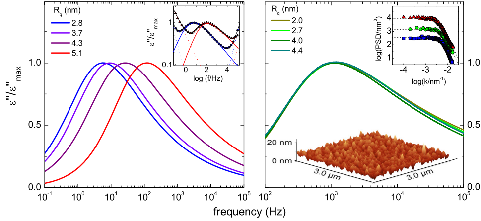
FIG. 1. Structural relaxation of 20 nm thin films of P4CIS at T = 412 K (left panel), and P2VP at T = 403 K (right panel) deposited on Al substrates of different roughness. To ease reading only the contribution of segmental mobility is given in the main panels, while in the inset of the left panel we plotted the raw dielectric signal of films of P4CIS on the smoothest and the roughest substrate, solid lines through the experimental data are fits to the HN function [29]. In the inset of the right panel, power spectral density of the surface of Al substrates (see an example of 3D view in the bottom of the panel) with different R_q values (blue squares 2 nm; green circles, 4 nm; red triangles, 9 nm) as a function of the wavelength k ; dashed lines are fits to the k -correlation, ABC function [13]. More details on fitting are provided in the Supplemental Material [25].
