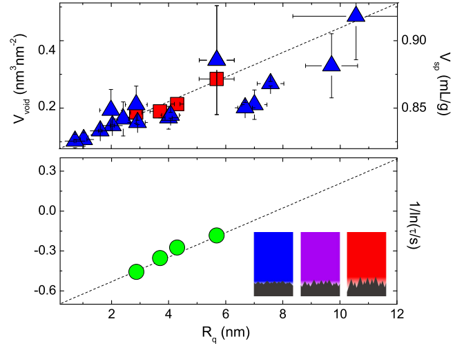
FIG. 3. Upper panel, the volume of voids determined via the Abbott method (blue triangles) and the specific volume of the polymer layer (red square) obtained via the CFV model are given as a function of the substrate roughness. Lower panel, the inverse of the segmental relaxation time is plotted as a function of the substrate roughness. Based on these results, we provided a series of sketches of the interface of a polymer with substrates of different roughness. By increasing R_q (left to right), the larger amplitude of the deviation from a flat substrate corresponds to a more pronounced reduction in density (pictured by less intense colors).
