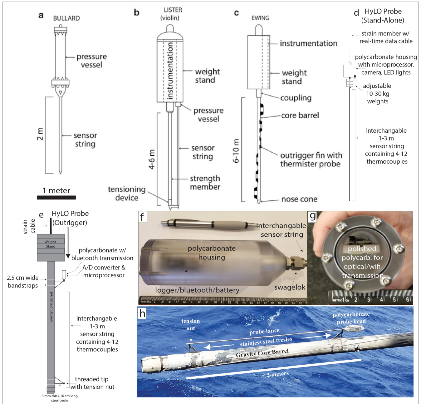
Figure 1. Mechanical configuration of the three most common marine heat flow probes (a,b,c) (Sclater et al., 2014) and the two HyLO Probe configurations (d, e). Photo images of the polycarbonate housing and join site of the probe head and lance for HyLO probes (f, g). Thermocouple strings are quickly interchangeable (~5 minutes) via swageloks (h). A photo of the first recovery of the HyLO probe outriggered to a 3-m-long gravity corer during sea trials from the R/V Meteor in May, 2019.
