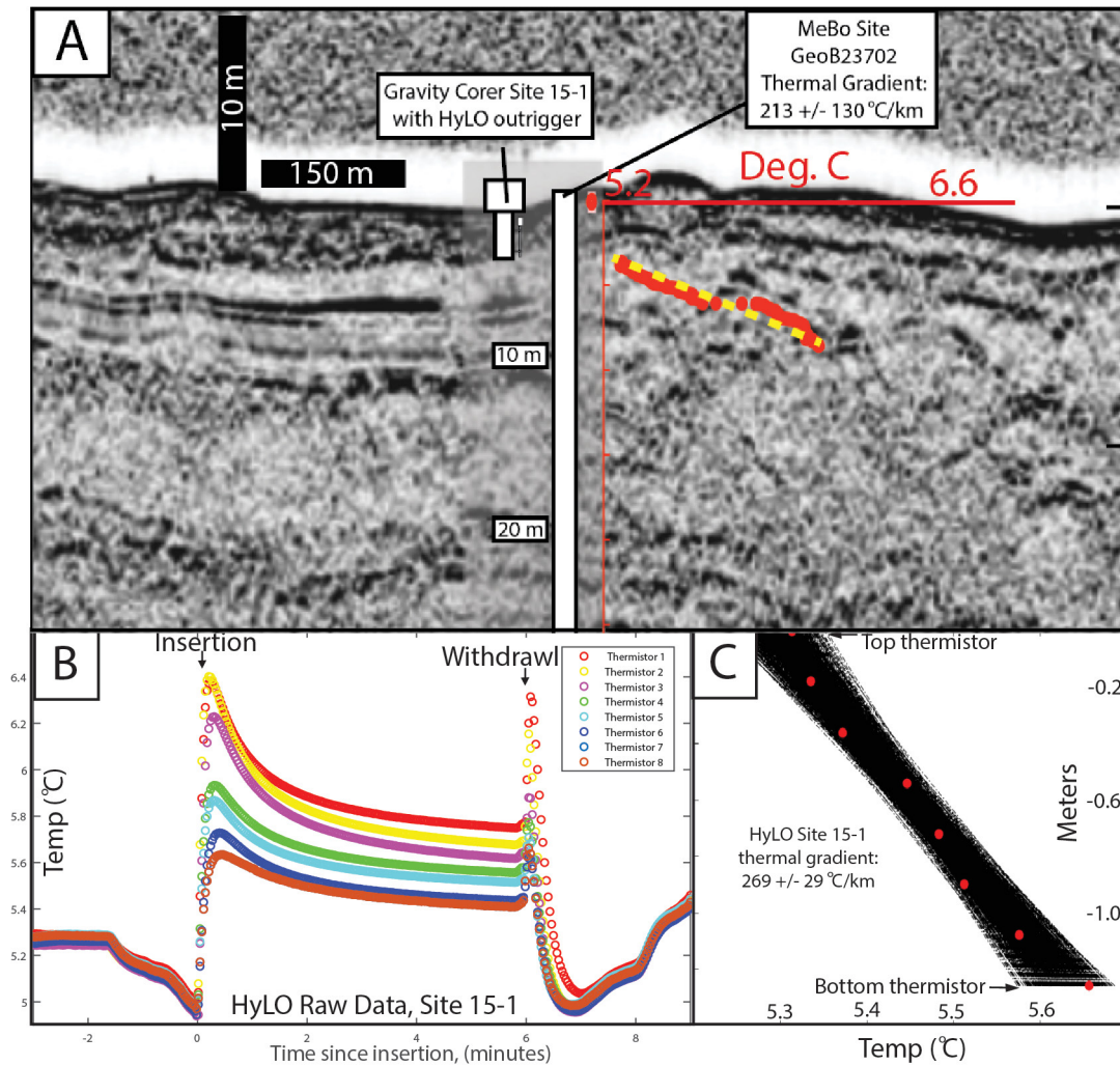
Figure 3. Comparison of thermal gradient measurements obtained from borehole temperature measurements with MeBo at depths of 5-to-9 mbsl versus the HyLO probe that measured thermal gradient in the upper 3 m of sediment. Parasound seismic data shows a cross-section of the subsurface and the location of HyLO gravity corer deployment within 50 m of MeBo drill site GeoB23702 (A). MeBo temperature measurements on the Acoustic borehole logging tool in figure 3A (red) indicate a high thermal gradient of approximately 213^\circ\text{C/km} (dashed yellow line) from 5 to 9 m below the sea floor. (B) There were 8 temperature recordings on the \sim 2 m long HyLO Probe that was outriggered to a 3-m-long gravity corer at Site 15-1, with thermocouples in the probe spaced \sim 0.18 m apart. Frictional heating observed both during probe insertion and withdrawal, as well as temperature decay for approximately 6 minutes after insertion indicate all 8 thermocouples penetrated the seafloor (B). Calculated steady-state temperature with depth (C) using the method of Villinger and Davis (1987) (red circles) that
