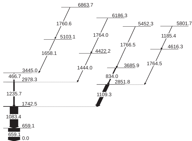
FIG. 4. Partial level scheme of ^{80}\text{Ge} showing the placement of four new transitions that make up the wide peak around 1764 keV. The widths of the arrows are proportional to the relative intensities of the \gamma -ray transitions.
