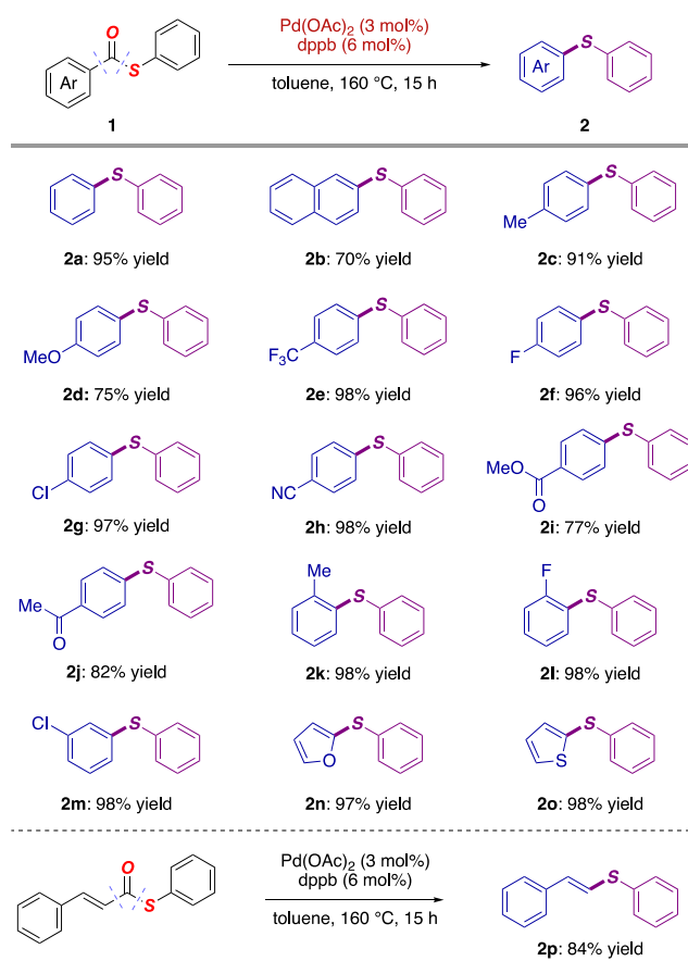
Scheme 1. Scope of Pd-Catalyzed General Intramolecular Decarbonylation of Thioesters.
