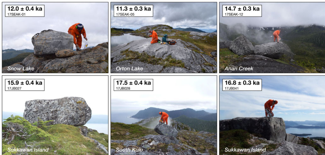
Figure 3. (color online) Examples of surfaces sampled for ^{10}\text{Be} dating. ^{10}\text{Be} ages are shown at 1 SD internal uncertainty. See online supplemental information for photographs of all samples.
