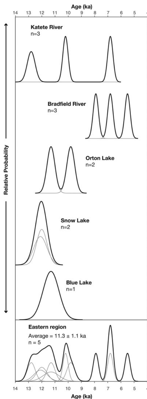
Figure 9. Normalized kernel density estimates for ^{10}\text{Be} ages in the eastern region of the study area. In the bottom panel, all ages from the eastern region are summed, and the average age for the eastern region excludes six young outliers.
