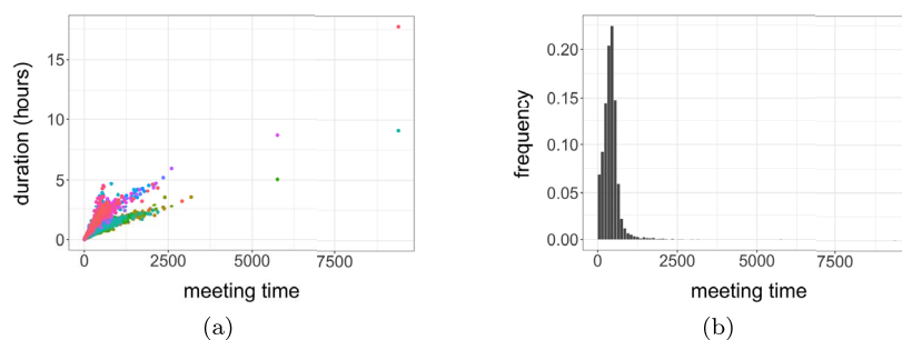
Fig 9: Left: duration (in hours) versus meeting times, using BPF with N = 4,096 particles. Each color corresponds to a different processor. Right: estimated histogram of the meeting times, in the neuroscience experiment of Section 4.2.
