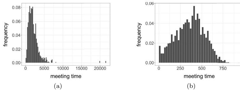
Fig 7: Histograms of meeting times associated with coupled PMMH chains, obtained with a standard deviation of the random walk proposal of 0.002 for a and 0.01 for \sigma_X^2 on the left, and with a larger standard deviation (0.01 on a and 0.05 on \sigma_X^2 ) on the right. In both cases, the likelihood was estimated with controlled SMC, with N = 128 particles, I = 3 iterations, in the neuroscience model of Section 4.2.
