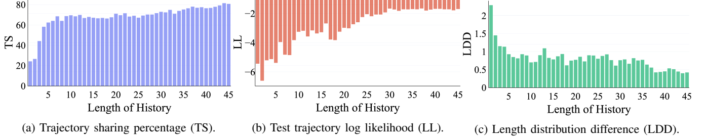
Fig. 5: The performances of GAIL_\ell over different length of history \ell 's.
