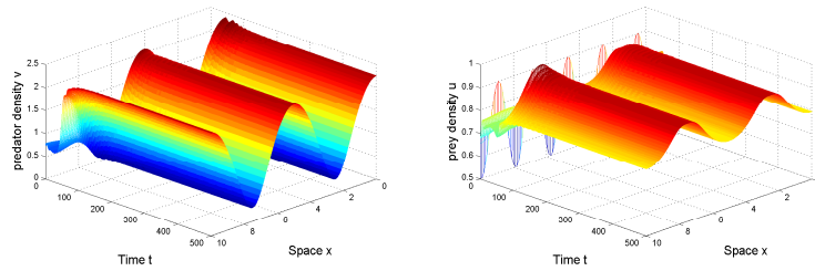
FIGURE 6. Instability induced by taxis in (25) when \xi = -0.5 and \eta = -0.4 and initial condition (0.7 + 0.1 \sin(2x), 0.7 + 0.2 \sin(3x)) . Other parameters are same as in Figure 4.
