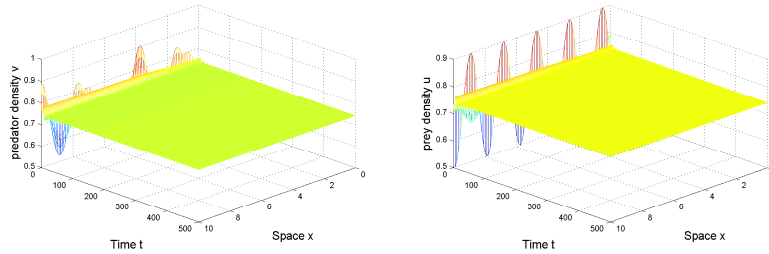
FIGURE 5. Turing pattern in (25) is stabilized when \xi = 0.9 and \eta = 0.4 , and the same initial value (0.7 + 0.1 \sin(2x), 0.7 + 0.2 \sin(3x)) . Other parameters are also same as in Figure 3.
