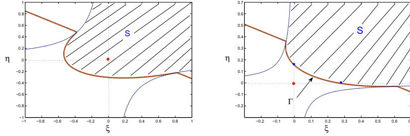
FIGURE 1. The stable region/unstable region of equilibrium (u^*, v^*) of system (1) in \xi - \eta parameter plane. Here f, g and other parameters are taken from (25) in Section 4. (Left): d = 0.06 , (0, 0) \in S ; (Right): d = 0.01 , (0, 0) \notin S . The thick solid curve is f_u + dg_v + \eta v^* f_v - \xi u^* g_u - 2\sqrt{d} + \xi \eta u^* v^* \sqrt{\text{Det} J} = 0 , the thin solid curve is d + \xi \eta u^* v^* = 0 in both panels.
