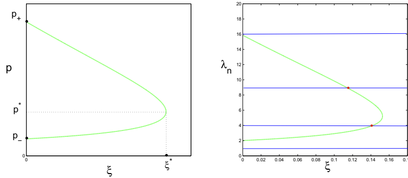
FIGURE 2. (Left): D(\eta, \xi, p) = 0 in \xi - p plane for fixed \eta ; (right): there are two bifurcation value \xi_S^2 (corresponding to \lambda_2 = 4 ) and \xi_S^3 (corresponding to \lambda_3 = 9 ), here f, g and other parameters are taken from (25) in Section 4 with \eta = 0.02 , d = 0.01 , \Omega = (0, \pi) .
