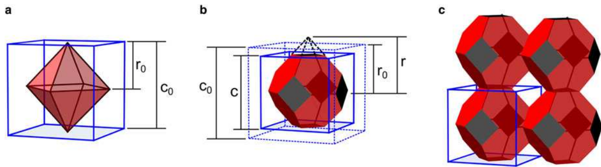
Fig. 6. Grain-scale model geometry. (a) Octahedron in the initial uncompressed and un-truncated state (red), enclosed by cubic cell lattice (blue). Cell size is the edge length c_0 , whereas the octahedron size is the half diameter r_0 . (b) Compressed cell and enclosed truncated octahedron. The enclosing cell is reduced in size from the initial c_0 (dotted blue) to c (solid blue), whereas the radius of the octahedron is enlarged ( r_0 up to r ) to allow the volume of the truncated octahedron to remain constant during compression. It is assumed that the truncated pyramidal mass (dashed black lines above the truncations) is transferred uniformly to the (red) octahedron faces. (c) Lattice of four octahedra showing stacking arrangement, connections and pores, in a compressed state. The model firn density of the illustrated arrangement is low ( 460 \text{ kg m}^{-3} ) to make the packing and geometry easier to view. A compressed cell is outlined surrounding the lower left firn grain.
