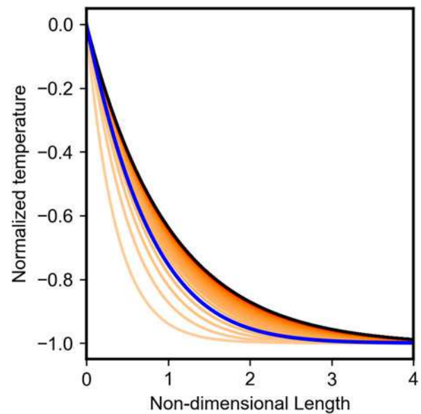
Fig. 7. Non-dimensional plot of the transient advection-diffusion temperature ahead of a moving water front. Length is normalized ( k_{firn}/v_{front} ), and temperature is normalized by initial firn temperature. In this moving reference frame (Lagrangian) plot, the x -axis translates to the right at the water front speed. Orange to black lines illustrate temperature evolution from initial (orange) to steady state (black). Steady state temperature is reached when the diffusion of heat from the water front is matched by the rate of advection of cold swept out by the advancing water front. Blue line is temperature at non-dimensional time of one.
