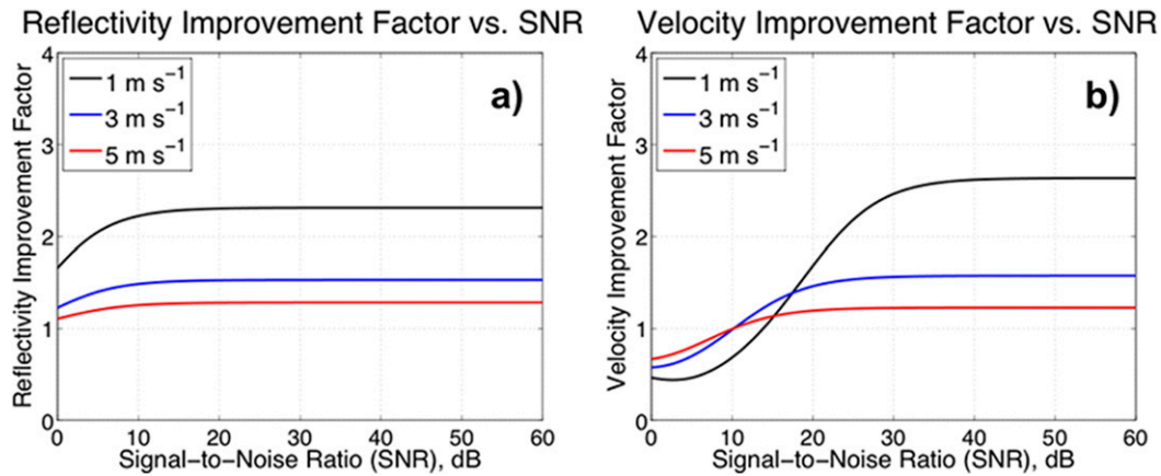
FIG. 1. Improvement factor for (a) Z_H and (b) v_r as a function of SNR using BMX. The three lines represent spectrum width of 1 (black line), 3 (blue line), and 5 \text{m s}^{-1} (red line).
