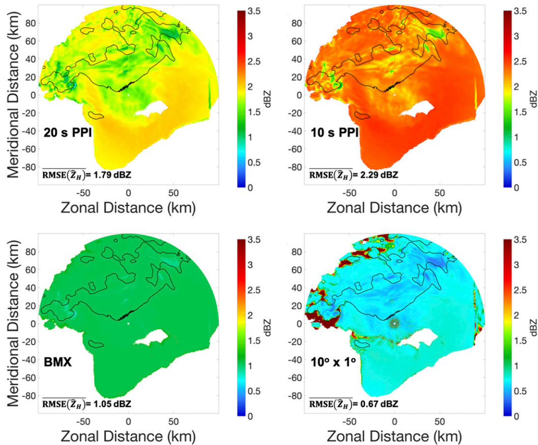
FIG. 7. As in Fig. 3, but for a longer radar standoff range ( \sim 60 km to the mesocyclone).
