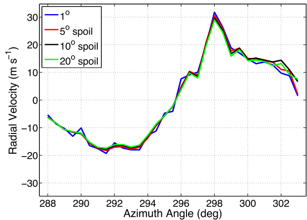
FIG. 13. The azimuthal radial velocity profile across the rotational couplet at 0.5^{\circ} in elevation (approximately 300 m AGL). Note that increasing the beam spoiling factor tends to decrease the measured \Delta V velocity shear.
