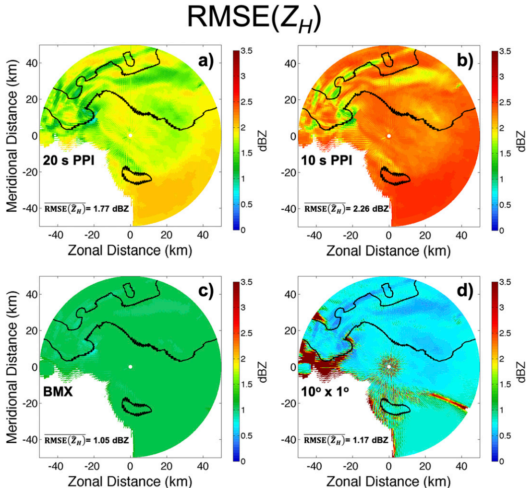
FIG. 3. PPIs showing the calculated RMSE of Z_H for (a) a pencil beam using CPS with a scan time of 20 s per PPI, (b) a pencil beam using CPS with a scan time of 10 s per PPI, (c) a pencil beam using BMX (IPS) with a scan time of 20 s per PPI, and (d) a 10° fan beam using CPS with a scan time of 20 s per PPI. All PPIs are at 0124:00 UTC, at 0.5° in elevation.
