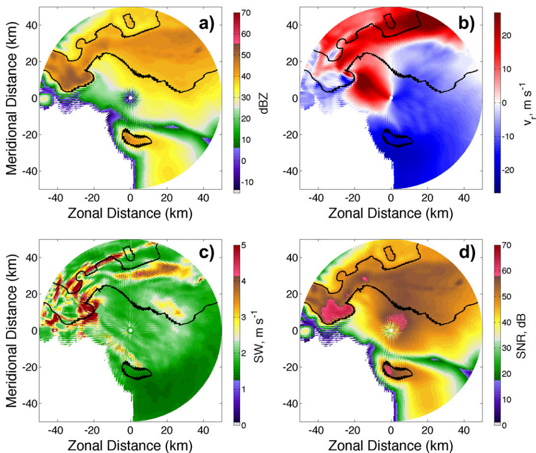
FIG. 2. PPIs showing (a) horizontal reflectivity factor ( Z_H , in dBZ), (b) radial velocity (in \text{m s}^{-1} ), (c) estimated spectrum width (in \text{m s}^{-1} ), and (d) signal-to-noise ratio (SNR; in dB). All PPIs are shown at 0124:00 UTC. Mean spectrum width is 2.48 \text{ m s}^{-1} . The black contour corresponds to 38 dBZ.
