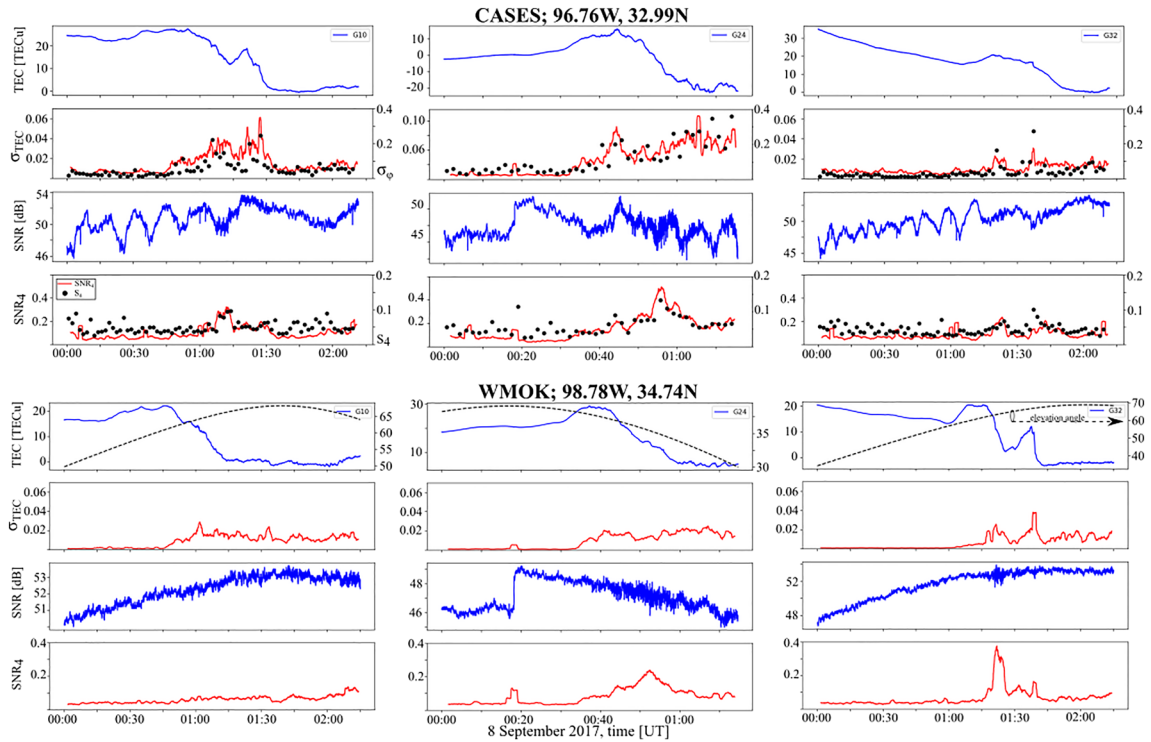
Figure 10. Comparison between observations taken by CASES (top) receiver from Dallas, TX, and wmok receiver from Oklahoma (bottom). Each row consists of three frames of data from G10, G24, and G32 satellites. Top row (CASES) has additional scintillation indices ( \sigma_\phi , S_4 ) in the second and bottom panels (respectively). Red lines represent the introduced ( \sigma_{TEC} , SNR_4 ) scintillation indices.
