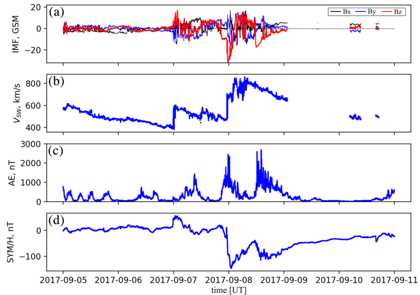
Figure 5. OMNIweb solar wind and geomagnetic indices from for the time period between 5 and 11 September 2017. (a) Interplanetary magnetic field components in Geocentric Solar Magnetospheric (GSM) coordinates. (b) Solar wind speed. (c) Auroral electrojet (AE) index. (d) Ring current strength proxy via SYM/H index.
