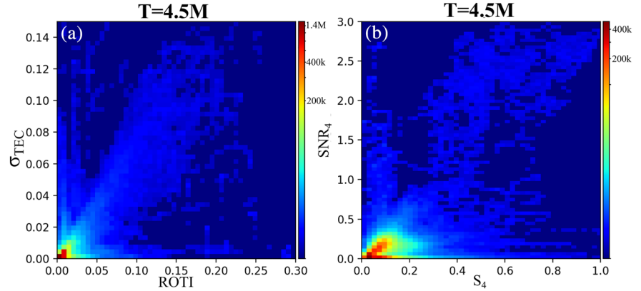
Figure 8. Two-dimensional histogram showing direct comparison between conventional and introduced scintillation indices, using data of six selected receivers from Table 1. The number of points is 4.5 million as shown in the title. (a) Comparison between ROTI and \sigma_{TEC} . (b) Comparison between S_4 and SNR_4 .
