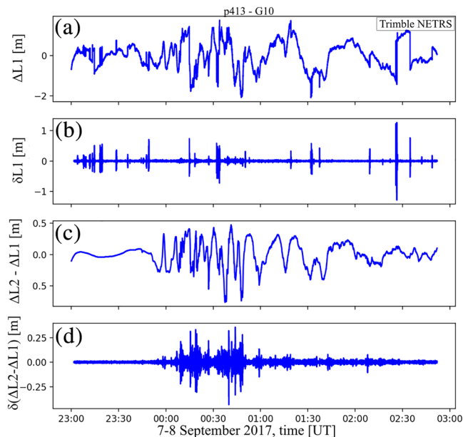
Figure 2. Carrier phase measurements (converted to range units) by the p413 receiver, measuring satellite G10, on 8 September 2017. (a) L1 detrended ( \Delta ) carrier phase. (b) High-pass filtered ( \delta ) L1 carrier phase. (c) Differential carrier phase measurements L2-L1. (d) High-pass filtered differential carrier phase of L2-L1.
