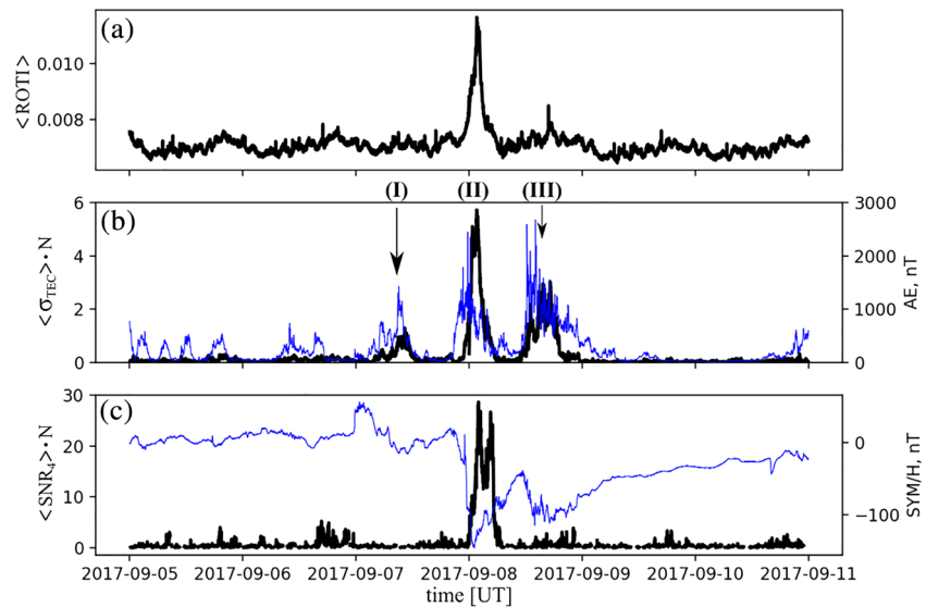
Figure 13. Scintillation indices time series plots from all available receivers, for the time period surrounding the 7–8 September geomagnetic storm. (a) ROTI time series represented by instantaneous median ( \langle \cdot \rangle ). (b) Median \sigma_{TEC} value normalized by total number of events N ( \langle \sigma_{TEC} \rangle \cdot N ). (c) Median SNR_4 value normalized by total number of instantaneous scintillation events N ( \langle SNR_4 \rangle \cdot N ).
