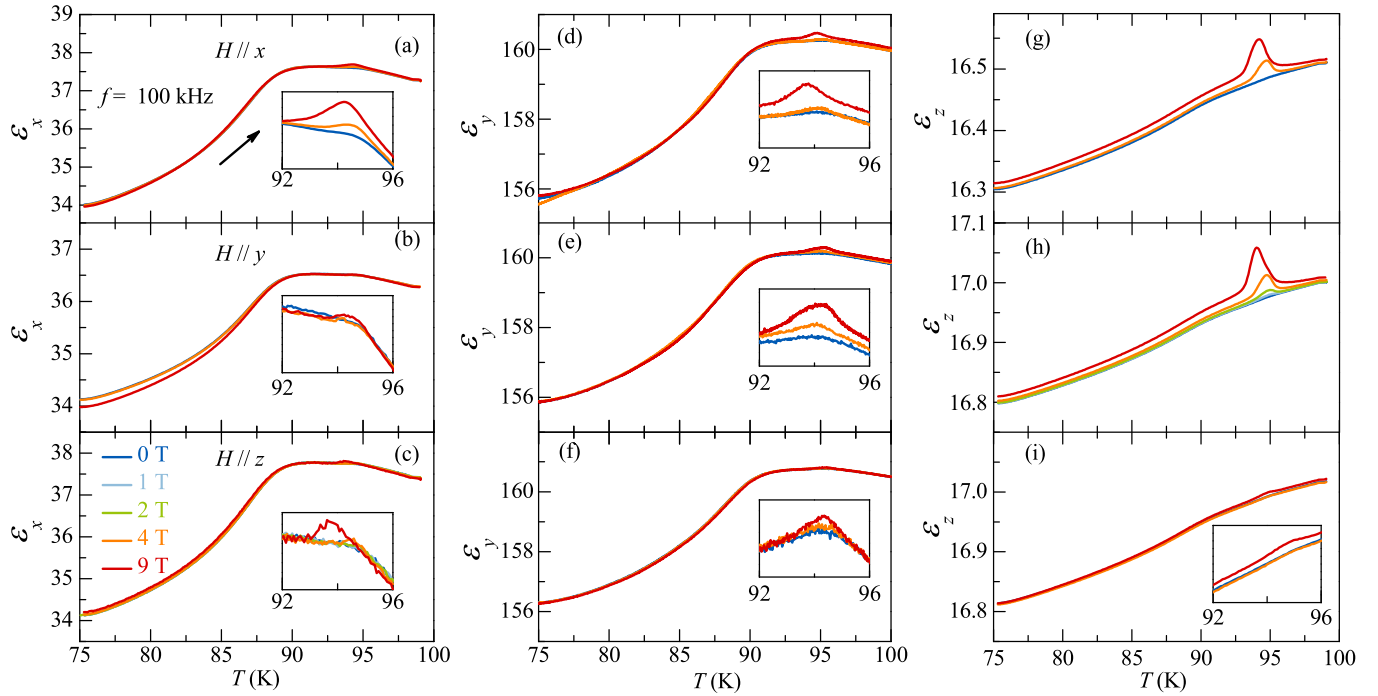
FIG. 2. The temperature-dependent relative dielectric constant of \text{Fe}_4\text{Nb}_2\text{O}_9 \epsilon_x for (a) H//x , (b) H//y , and (c) H//z , \epsilon_y for (d) H//x , (e) H//y , and (f) H//z , and \epsilon_z for (g) H//x , (h) H//y , and (i) H//z . All the data are measured in warming. Insets of (a)–(f) and (i) show the data around 94 K.
