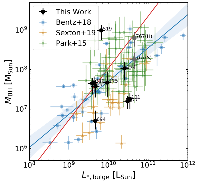
Figure 5. BH mass as a function of bulge luminosity (all in the V band, except for Sexton et al. 2019 in the SDSS- r band). The blue line shows the best fit (with 1\sigma scatter shown in the blue shaded area) from the Bentz & Manne-Nicholas (2018) sample and red line shows the best fit from the local sample of Kormendy & Ho (2013).
