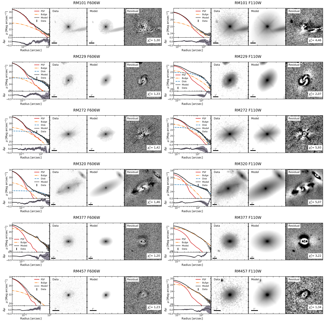
Figure 1. Surface brightness decomposition of all sources in the F606W and F110W bands. The left panel is the surface brightness profile of the data (black dots), the model (gray solid line), and each modeled component (red solid lines for PSFs, orange dotted-dashed lines for hosts/bulges ( n = 4 ), blue dash lines for exponential disks ( n = 1 ), and purple dotted lines for truncated rings (RM775 only)). The radial profiles are directly measured from the GALFIT decomposed models and the HST images with isophote fitting. The bottom sub-panel (in the leftmost panel) is the residual of the surface brightness profile, with rms along the elliptical path plotted in gray shaded area. The right three images are (from left to right) the HST image, the GALFIT model and the residual. The residual images display the first to 99th percentiles (with linear stretch) of the residual values to provide better visual contrast. The reduced \chi^2 of the model is labeled in the lower right corner of the residual image.
