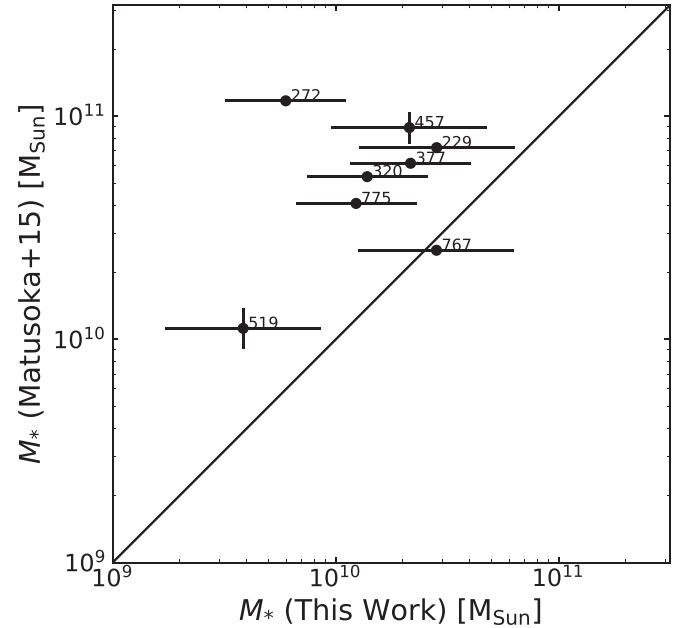
Figure 7. Comparison of the derived host mass from this work and Matsuoka et al. (2015). The black solid line is the 1:1 line for guidance.
