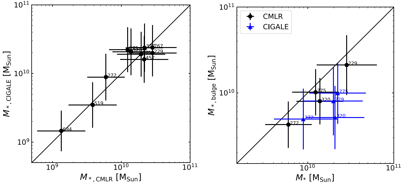
Figure 3. Left: comparison of host stellar masses derived from color- M_*/L relations (CMLRs) and CIGALE. Right: comparison of the total host stellar mass and bulge mass derived from CMLRs and CIGALE. The black solid lines are the 1:1 lines.
