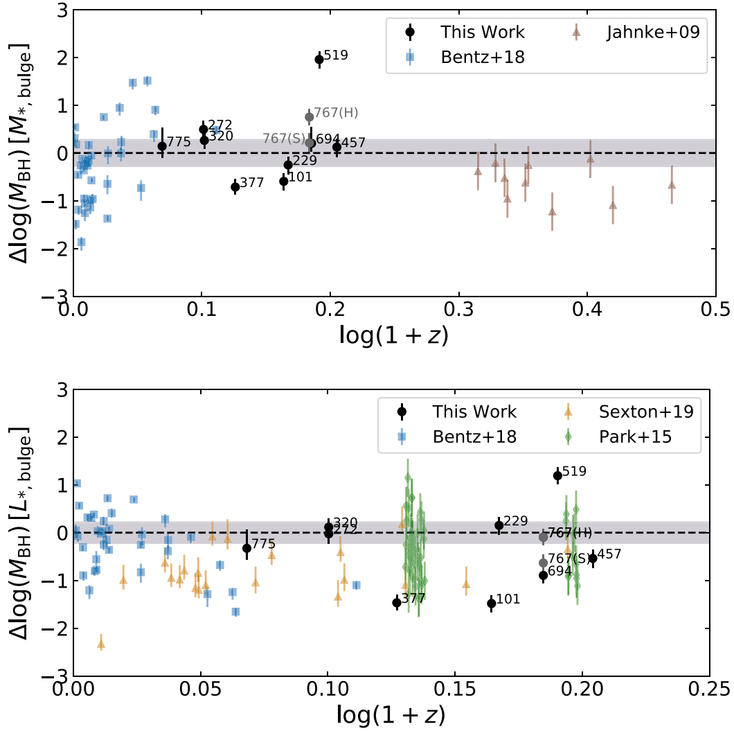
Figure 8. Evolution of \Delta \log(M_{\text{BH}}) with redshift, with baselines adopted from the best-fit relations of M_{\text{BH}}-M_{*,\text{bulge}} and M_{\text{BH}}-L_{*,\text{bulge}} from the Kormendy & Ho (2013) sample. Vertical error bars are from uncertainties in BH mass only.
