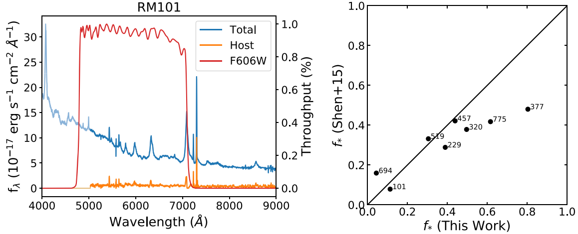
Figure 6. Comparison of spectral decomposition and image decomposition in the estimation of host fraction in quasars. Left: HST F606W filter overlaid on the total and decomposed (host-only) spectra from Shen et al. (2015a) in observed wavelength. We only compute the stellar fraction in the spectral range covered by both the total and decomposed spectral, as shown in the thick solid lines. Right: comparison of the derived stellar fraction from this work and Shen et al. (2015a) in the F606W bandpass. The black dashed line shows the 1:1 ratio line.
