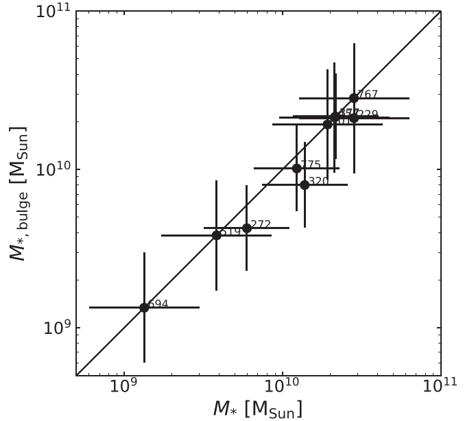
Figure 2. Comparison of the stellar masses of the host galaxy (total host mass) and the bulge component. The black solid line is the 1:1 line for guidance.
