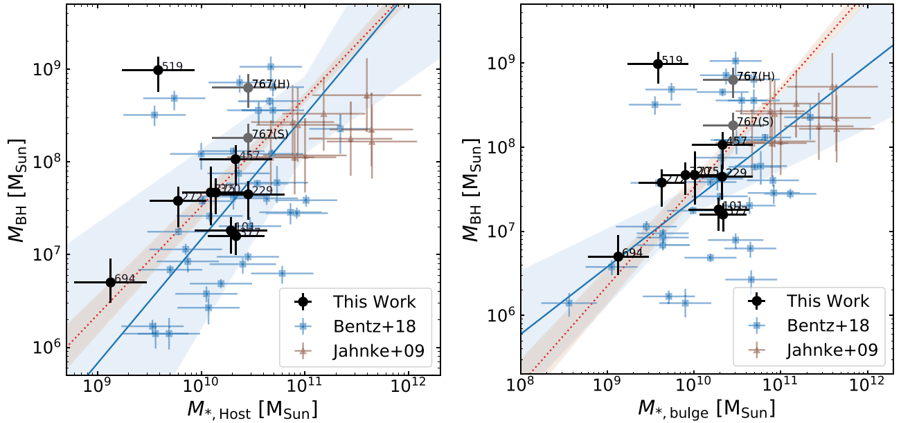
Figure 4. Black hole (BH) mass as a function of the host-galaxy mass (left) and bulge mass (right). The blue points are the local-reverberation mapping (RM) sample from Bentz & Manne-Nicholas (2018), and their best-fit relations and 1\sigma scatter are shown with blue solid lines and the blue shaded area. The red line denotes the best fit (with 1\sigma scatter in red shaded region) of the BH mass–bulge mass relation of the local quiescent galaxy sample from Kormendy & Ho (2013). For RM767 (gray points), we plot the RM-based BH masses using lags measured from both (Shen et al. 2016, labeled with S) and (Homayouni et al. 2020, labeled with H).
