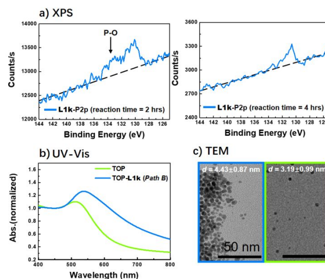
Figure 2. a) P2p XPS spectra of L1k capped AuNPs synthesized in 2 hrs and 4 hrs via Path B . b) UV-Vis spectra of TOP ( L1c , green) and L1k (blue) capped AuNPs. c) TEM images of TOP ( L1c , green), and L1k (blue) capped AuNPs.
