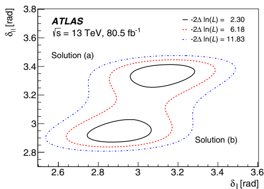
Fig. 9 Two-dimensional constraints on the values of \delta_{||} and \delta_{\perp} for solutions (a) and (b) at the level of -2\Delta\ln(L) = 2.30, 6.18 , and 11.83 respectively created using a full 2D scan. The minimum of the solution (b) is -2\Delta\ln(L) = 0.03 higher than the minimum of the solution (a)
