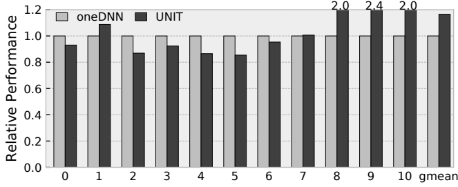
Fig. 13: The performance of each layer on res18-3d.
