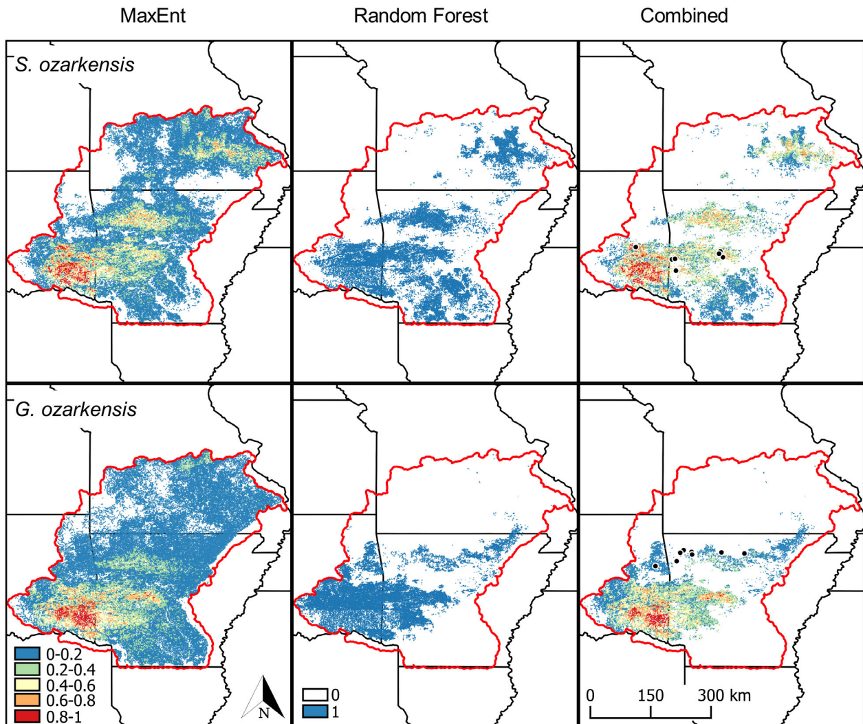
Figure 2. Stream level predictions of both focal species. MaxEnt-only, Random Forest-only, and combined model predictions are presented as probability of presence (0–1) represented by colour classifications from low probability, Blue (0–0.2) to high probability, Red (0.8–1). Ozark-Ouachita Interior Highlands region outlined in red. New detections discovered through field surveys of each species are shown with black points. [Color figure can be viewed at wileyonlinelibrary.com ]
