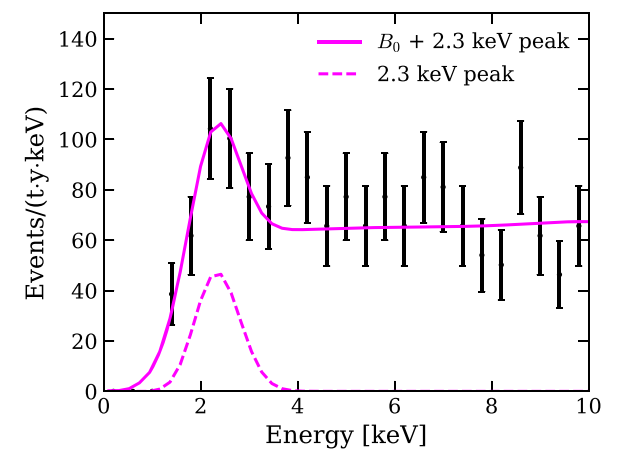
FIG. 11. Left: the log-likelihood ratio q for different bosonic dark matter masses with respect to the best-fit mass at 2.3 keV/c 2 . At each mass, we show the result for the corresponding best-fit coupling. The green band shows an asymptotic 68% C.L. confidence interval on the bosonic dark matter mass. The local significance for each mass is indicated by the right y-axis. Right: best fit of a 2.3 keV peak and B_0 to the data. A 0.4 keV binning is used for better visualization.
