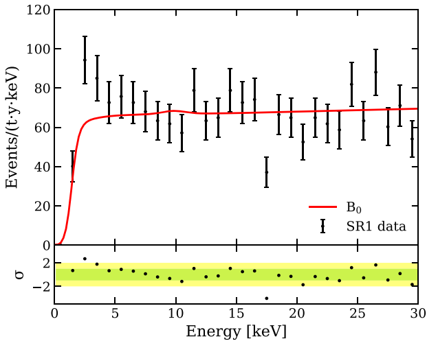
FIG. 4. A zoomed-in and rebinned version of Fig. 3 (top), where the data display an excess over the background model B_0 . In the following sections, this excess is interpreted under solar axion, neutrino magnetic moment, and tritium hypotheses.
