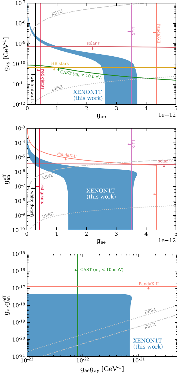
FIG. 8. Constraints on the axion-electron g_{ae} , axion-photon g_{ay} , and effective axion-nucleon g_{an}^{\text{eff}} couplings from a search for solar axions. The shaded blue regions show the two-dimensional projections of the three-dimensional confidence surface (90% C.L.) of this work and hold for m_a < 100 \text{ eV}/c^2 . See text for more details on the three individual projections. All three plots include constraints (90% C.L.) from other axion searches, with arrows denoting allowed regions, and the predicted values from the benchmark QCD axion models DFSZ and KSVZ.
