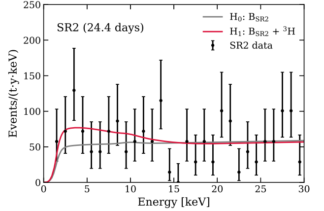
FIG. 12. A fit to SR2 data if tritium is treated as a signal. The red (gray) line is the fit with (without) tritium in the background model.
