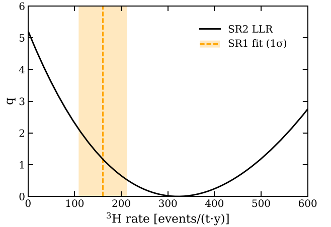
FIG. 13. The log-likelihood ratio curve for the tritium rate in SR2. The orange line and band indicate the best fit and 1\sigma uncertainty for the tritium rate in SR1. The SR2 fit result is consistent with SR1, but with a large uncertainty due to limited statistics.
