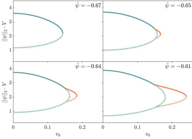
FIG. 12. A sequence of bifurcation diagrams \|\psi\|_2 vs v_0 showing how traveling one-peak LS (orange line) come into existence with increasing mean density \bar{\psi} (from top left to bottom right) at \epsilon = -0.98 (corresponding to the value used in [38]). Two drift-pitchfork bifurcations appear simultaneously at the saddle-node bifurcation of the branch of resting LS (blue line). Increasing \bar{\psi} further expands the range of existence of traveling LS toward larger v_0 and the drift-pitchfork bifurcations separate. The onset of motion is always at v_c \approx 0.15 . Remaining line styles, parameters, and the domain size are as in Fig. 5.
