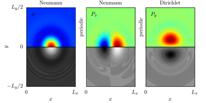
FIG. 1. Sketch of the numerical setup: Two-dimensional structures that are reflection symmetric with respect to the x axis are computed on a reduced domain [0, L_x] \times [0, L_y/2] as indicated by the colored area. The density field \psi and the x -component P_x of the polarization satisfy Neumann boundary conditions at y = 0 while Dirichlet boundary conditions apply to the y -component P_y of the polarization: P_y = 0 at y = 0 . All fields are periodic in the x direction, i.e., only motion in the x direction is allowed. For visualization, the entire domain \Omega_{\text{exp}} = [0, L_x] \times [-L_y/2, L_y/2] , indicated by the colored and grayscale regions, is used.
