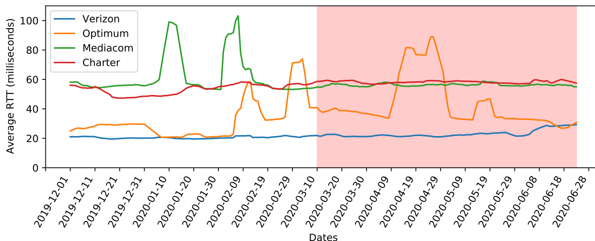
(a) 95th percentile of ISP latency (Group 1).
