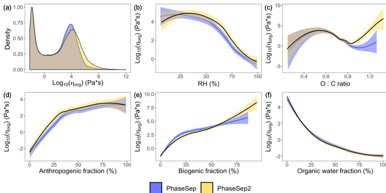
Figure 4. For all grid cells and time steps at the surface layer, the (a) probability distribution of the organic-phase viscosity and correlations of particle viscosity ( \eta_{\text{org}} ) with (b) relative humidity, (c) atomic oxygen to carbon (O : C) ratio, (d) anthropogenic SOA weight fraction, (e) biogenic SOA weight fraction and (f) organic-phase water content ( w_s ) for PhaseSep (blue) and PhaseSep2 (gold).
