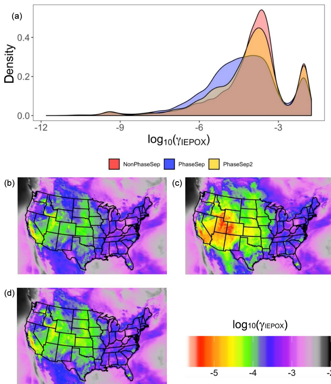
Figure 7. For all grid cells and time steps, the predicted (a) probability distribution of \gamma_{\text{IEPOX}} at the surface level for the NonPhaseSep (red), PhaseSep (blue) and PhaseSep2 (gold) simulations. For each grid cell, the mean value of \gamma_{\text{IEPOX}} for the (b) NonPhaseSep, (c) PhaseSep and (d) PhaseSep2 simulations.
