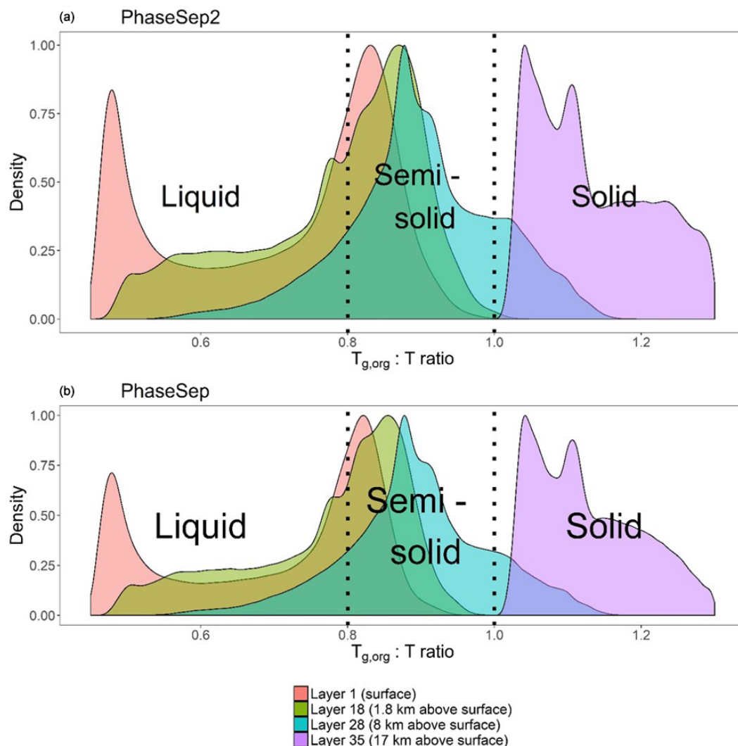
Figure 1. Probability density distribution of glass transition temperature to ambient temperature ratio ( T_{g,org} : T ) for all grid cells and time steps for (a) the PhaseSep2 simulation and (b) the PhaseSep simulation at the surface layer (red), lower troposphere (green), upper troposphere (blue) and stratosphere (purple).
