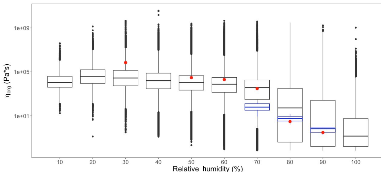
Figure 6. Model-predicted SOA viscosity ( \eta_{\text{org}} ) and experimental data for \eta_{\text{org}} from Y. Zhang et al. (2018) (red) and Song et al. (2016) (blue) at varying RH.
