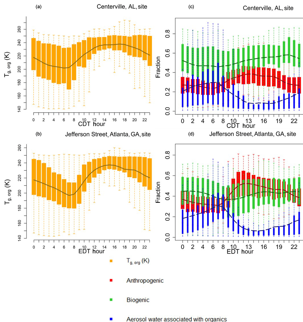
Figure 3. Diurnal pattern for SOAS (1 June–15 July) 2013 of the organic glass transition temperature ( T_{g,org} – orange), and contributions of anthropogenic OA (red), biogenic OA (green) and aerosol water associated with organics (blue) to T_{g,org} in the PhaseSep2 case at the (a, c) Centerville, AL, site and the (b, d) Jefferson Street, Atlanta, GA, site. Bars/shaded boxes indicate 25th to 75th percentiles. Extreme bounds of whiskers indicate 5th to 95th percentiles (i.e., 95 % confidence interval), and the line indicates the mean.
