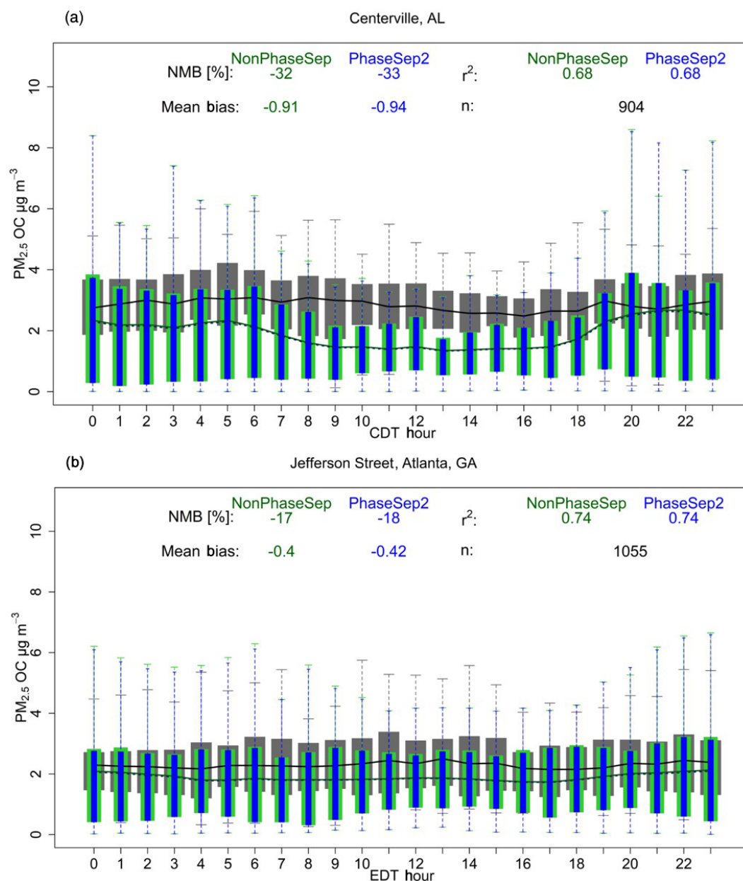
Figure 9. PM 2.5 organic carbon (OC) mass ( \mu\text{g m}^{-3} ) as a function of hour of the day. Non-aggregated performance statistics – mean bias ( \mu\text{g m}^{-3} ), % normalized mean bias (NMB) and Spearman’s correlation coefficient ( r^2 ) of NonPhaseSep (green) and PhaseSep2 (blue) cases relative to observed (grey) PM 2.5 OC mass for the (a) rural Centerville, AL, site and (b) urban Jefferson Street, Atlanta, GA, site. Bars/shading indicate 25th to 75th percentiles. Extreme bounds of whiskers indicate 5th to 95th percentiles (i.e., 95 % confidence interval). Lines indicate means (dashed line indicates PhaseSep2). n is the number of observation points.
