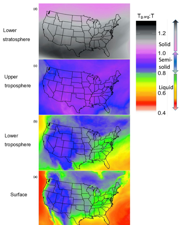
Figure 2. For all time steps and over the continental United States, the average glass transition temperature to ambient temperature ( T_{g,org} : T ) ratio at (a) the surface level, (b) 1.8 km above the surface layer (lower troposphere), (c) 8 km above the surface layer (upper troposphere) and (d) 17 km above the surface layer (stratosphere) for the PhaseSep2 simulation.
