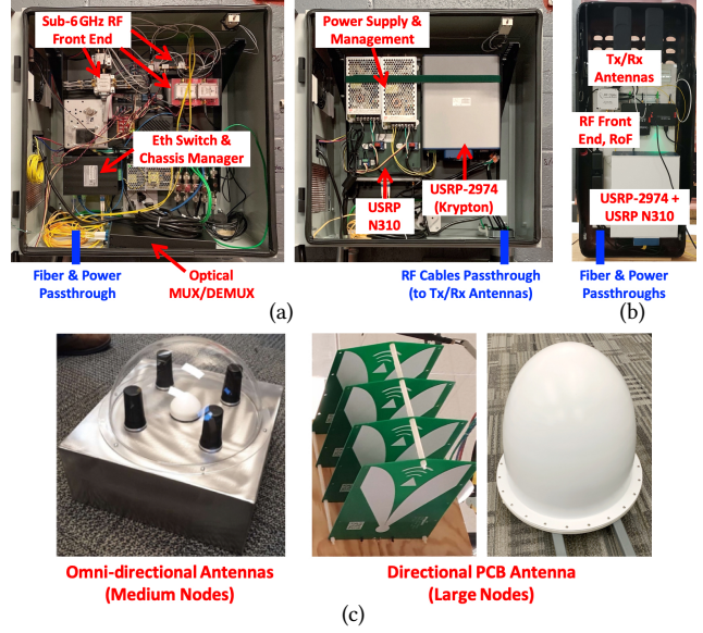
Figure 4: (a) Developed and deployed medium node (or a large node) with the components mounted on the top shelf (left) and bottom (right) shelf, (b) prototype of the light version of the medium node for lightpole mounting ( medium-light ) with the components layout, and (c) sub-6 GHz wideband antennas used for the medium (left) and large (right) node.
