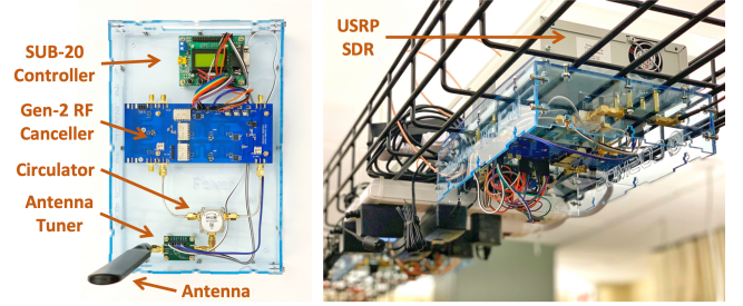
Figure 12: The 2 nd -generation wideband full-duplex radio [85] (left) and its integration in the COSMOS testbed sandbox (right) allowing for remote access and compute through COSMOS’ optical network [84].
