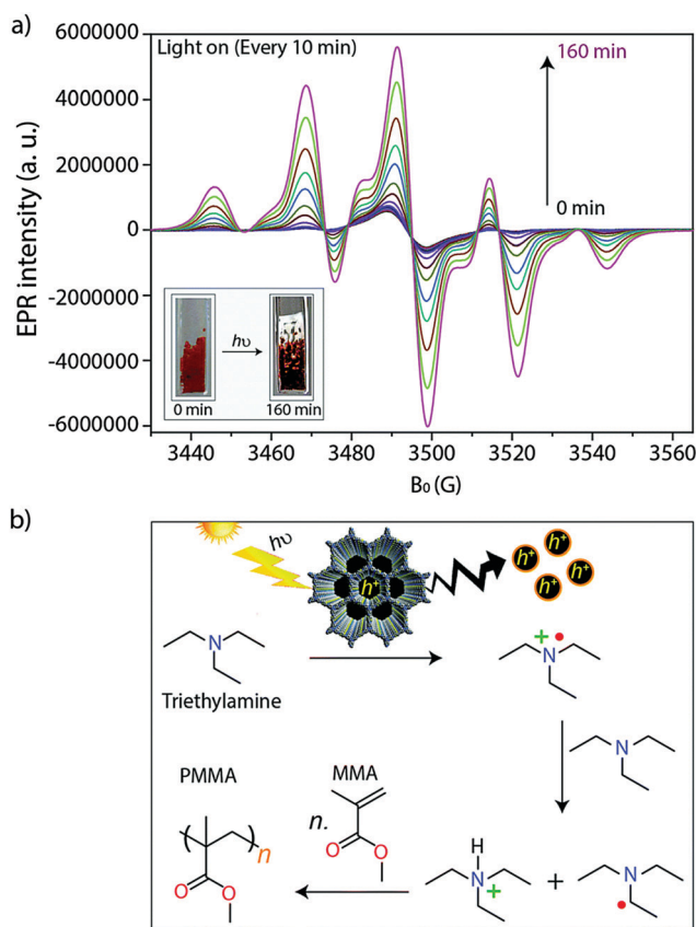
Fig. 28 (a) In situ EPR spectra during the photocatalyzed free radical polymerization of MMA to PMMA. (b) Proposed mechanism for the TTT-BDTA catalyzed conversion of MMA to PMMA. Reproduced from Chem. Sci. , 2019, 10 , 8316–8322, with permission from the Royal Society of Chemistry.
