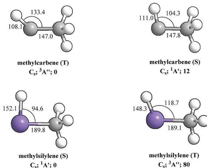
Scheme 2. Molecular structures, point groups, relative energies (kJ mol -1 ), bond distances (pm), and selected bond angles (degrees) for triplet and singlet methylcarbene (CH 3 CH) and methylsilylene (HSiCH 3 ). Carbon, silicon, and hydrogen are color coded in gray, purple, and white, respectively.
