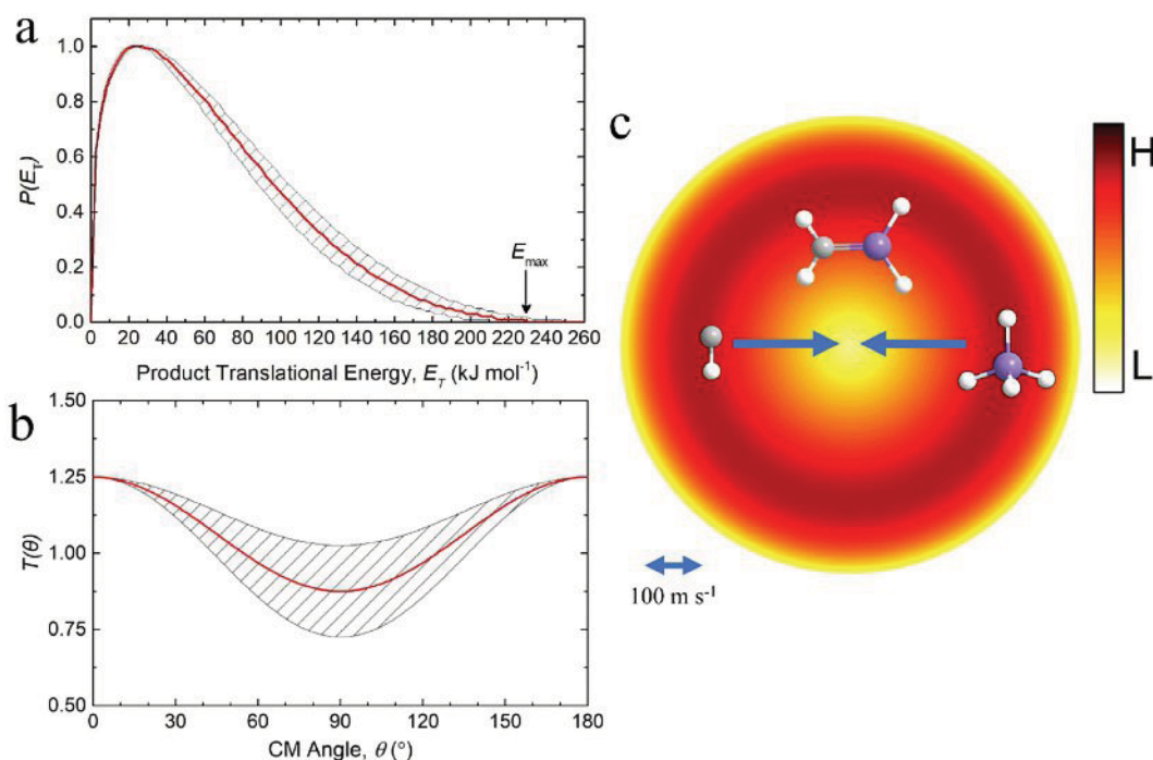
Figure 2. Center-of-Mass (CM) distributions and the associated flux contour map. CM translational energy flux distribution (a), CM angular flux distribution (b), and the top view of their corresponding flux contour map (c) leading to the formation of silene ( \text{H}_2\text{SiCH}_2 ) plus atomic hydrogen in the reaction of methylidyne with silane. Shaded areas indicate the error limits of the best fits accounting for the uncertainties of the laboratory angular distribution and TOF spectra; the red solid lines define the best-fit functions. Carbon, silicon, and hydrogen are color coded in gray, purple, and white, respectively.
