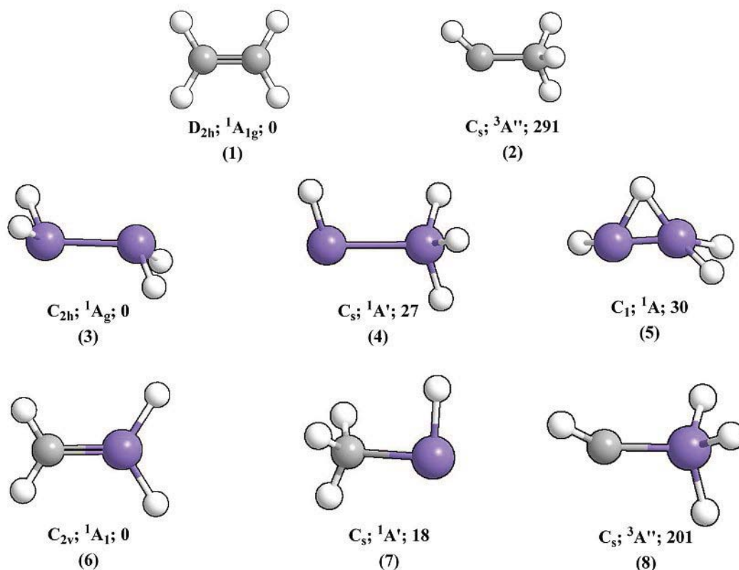
Scheme 1. Structures, point groups, electronic ground state wave functions, and relative energies (kJ mol -1 ) of homo- and heteronuclear tetrahydrides of main group XIV elements involving carbon (gray) and silicon (purple) with hydrogen atoms color coded in white.
