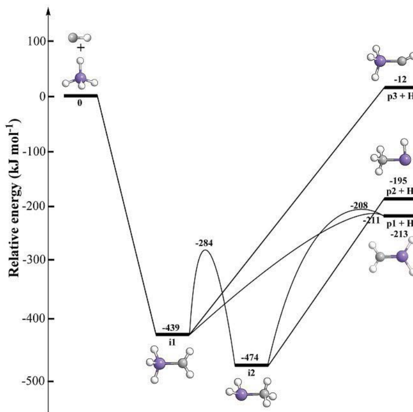
Figure 3. Potential energy surface for the reaction of the methylidyne radical with silane involving atomic hydrogen loss pathways. Cartesian coordinates of the atoms vibrational frequencies are compiled in Table S3; a complete potential energy surface including the molecular hydrogen loss pathways is presented in Figure S1. Carbon, silicon, and hydrogen are color coded in gray, purple, and white, respectively.
