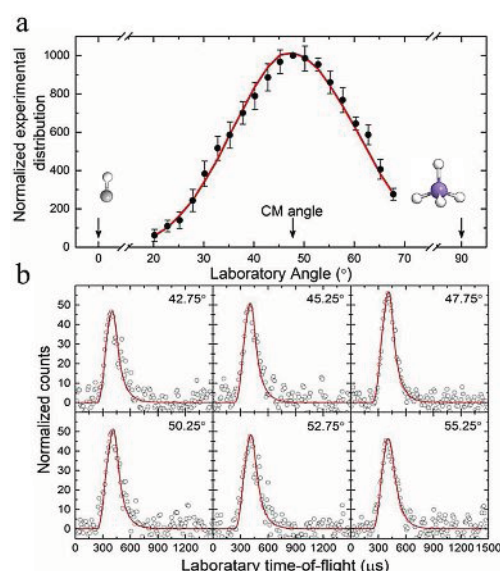
Figure 1. Laboratory angular distribution and the associated time-of-flight spectra. Laboratory angular distribution at mass-to-charge ratio ( m/z ) of m/z = 43 recorded in the reaction of the methylidyne radical with silane (a), and the time-of-flight spectra recorded at distinct laboratory angles overlaid with the best fits (b). The solid circles with their error bars represent the normalized experimental distribution with \pm 1\sigma uncertainty; the open circles indicate the experimental data points of the time-of-flight spectra. The red lines represent the best fits obtained from the optimized center-of-mass (CM) functions, as depicted in Figure 2. Carbon, silicon, and hydrogen are color coded in gray, purple, and white, respectively.
