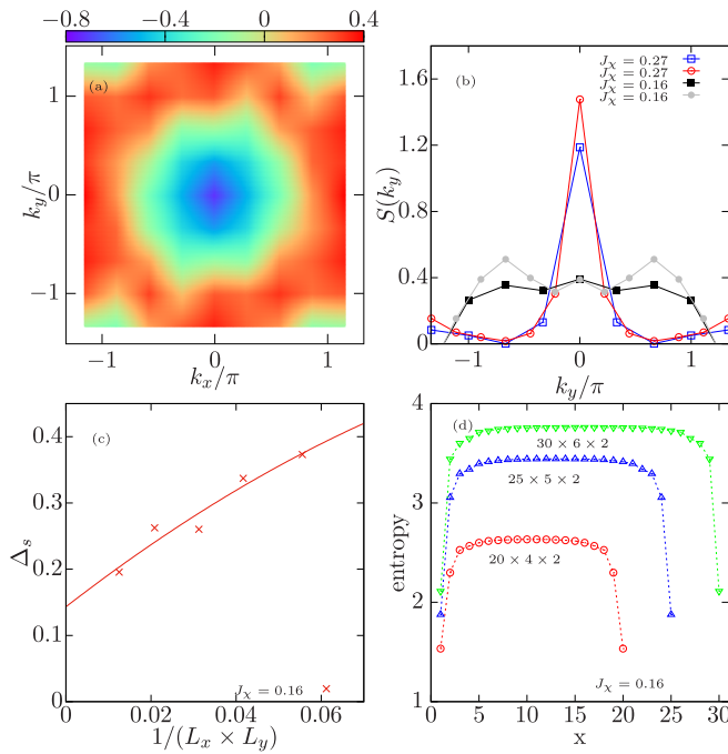
FIG. 4. (a) refers to the spin structure in the CSL phase at J_2 = 0.2 , J_\chi = 0.16 where there is no peak as opposed to other magnetic phases. This result is based on the cluster of 20 \times 4 \times 2 . (b) refers to the spin structure peaks with fixed k_x = -\frac{2\pi}{\sqrt{3}} of various parameters. The blue and red lines are obtained in the chiral spin state with clusters of 20 \times 4 \times 2 and 30 \times 6 \times 2 , respectively. The magnitude of the peak increases as the cluster size increases. The black and gray lines are obtained in the CSL with the same two clusters, where there is no significant peak. (c) refers to the finite size scaling of the spin gap on the torus geometry with clusters of 3 \times 3 \times 2 , 4 \times 3 \times 2 , 4 \times 4 \times 2 , 6 \times 4 \times 2 , and 8 \times 5 \times 2 . (d) refers to the entanglement entropy with various clusters on finite cylinders in the CSL phase. The x here denotes the distance of the cut in the x direction. All of the results are obtained at J_2 = 0.2 .
