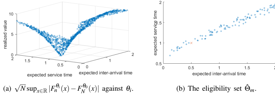
Figure 2: Apply Algorithm 1 to calibrate (\lambda, \mu) .
