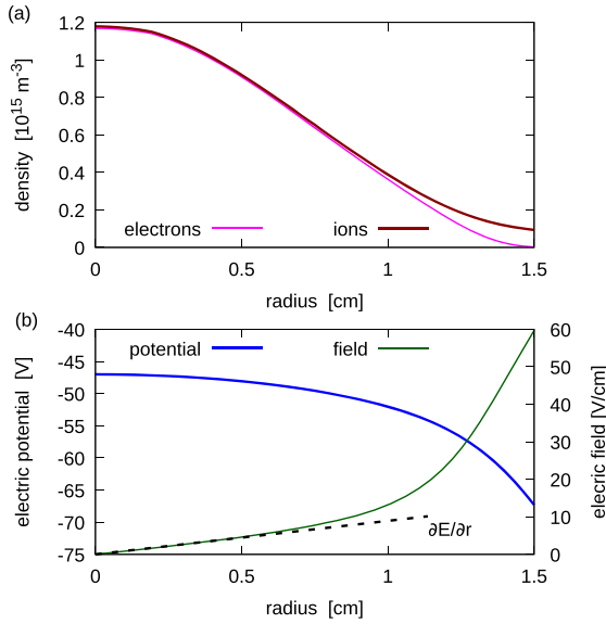
Figure 9. Time averaged radial distribution of (a) electron and \text{Ne}^+ ion densities and (b) the electric potential and radial electric field in the positive column at p = 60 Pa, I = 2 mA, and x = 200 mm. The dashed straight line represents a linear fit to the radial electric field in the bulk center ( r < 5 mm).
