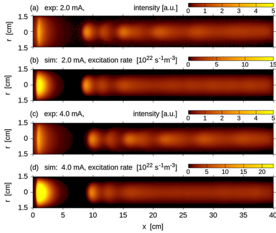
Figure 2. Experimental (a) and (c) light intensity distributions and computed (b) and (d) line-of-sight integrated (Abel transformed) total excitation distribution functions. The discharge pressure is p = 60 Pa, the currents are indicated in the panel labels, and the cathode is at x = 0 facing the anode at x = 400 mm. The exposure (40 ms) and numerical data acquisition times (1 ms) were chosen to be long enough to represent the time-averaged stationary states. Intensity values are normalized to cover the full color scale in all panels. Here and in all similar figures to come the real aspect ratio of 3:40 is scaled by stretching the radial axis by a factor of two for better visibility.
