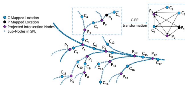
Figure 2. Illustration of a localized river network subset from the entire network with contaminant (noted as “C”) and polluter (noted as “P”) locations shown individually. Inset shows C-PP transformation over a subnetwork that was based on directed river flow. For the polluting spill P_1 , C_1 is the only Type I upstream samples while, for example, C_7 and C_4 are Type II background samples.
