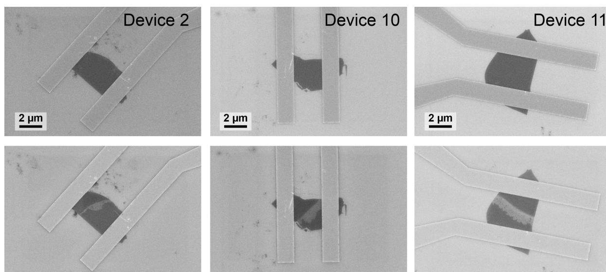
Figure S2. SEM images of selected \text{Ti}_3\text{C}_2\text{T}_x devices before (top row) and after (lower row) current breakdown.
