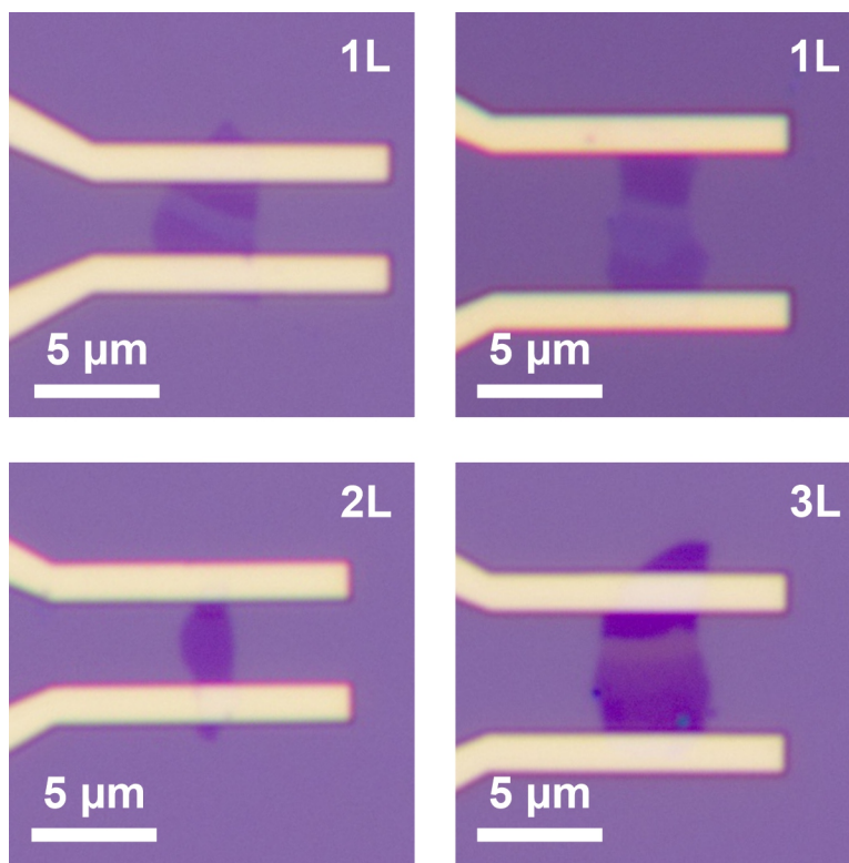
Figure S3. Optical images of selected \text{Ti}_3\text{C}_2\text{T}_x devices after current breakdown.
