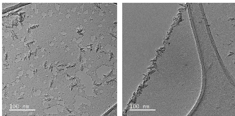
Figure S1. TEM images of representative degraded \text{Ti}_3\text{C}_2\text{T}_x flakes showing the formation of nanoscopic holes and \text{TiO}_2 particles that primarily aggregate near the edges. Higher quality \text{Ti}_3\text{C}_2\text{T}_x flakes that did not exhibit these features (Figure 1G) were used for device fabrication and electrical measurements.
