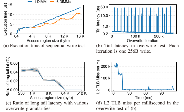
Fig. 7. LENS policy prober tests on Optane DIMM.
