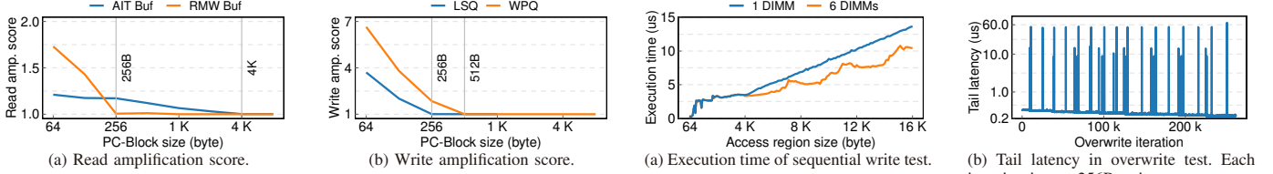
Fig. 6. Read(a) and write(b) amplification scores in our buffer prober test.
