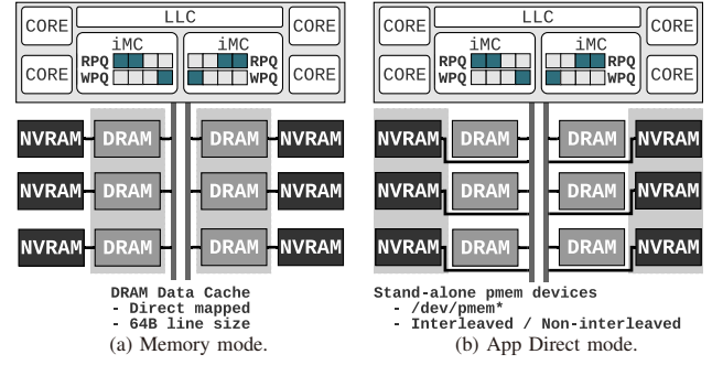
Fig. 2. Optane DIMM-based system configurations.
