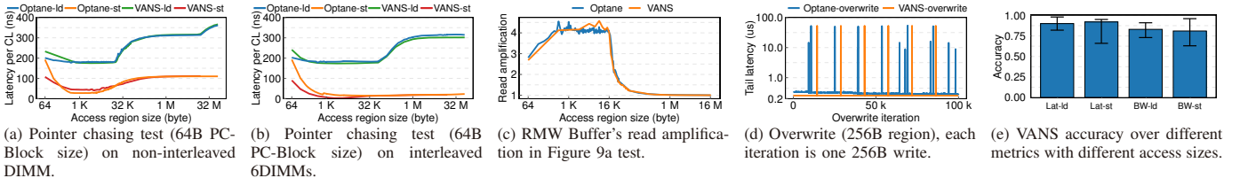
Fig. 9. VANS performance validation with microbenchmarks: (a-c) pointer chasing and (d) overwrite. (e) VANS overall accuracy on load/store latency and bandwidth.
