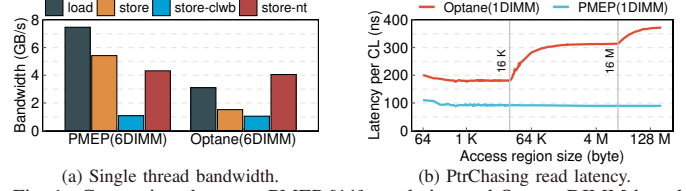
Fig. 1. Comparison between PMEP [11] emulation and Optane DIMM-based real machine measurement. Store-clwb are writes followed by clwb cache write-back instructions [20]; store-nt are non-temporal writes [20].
