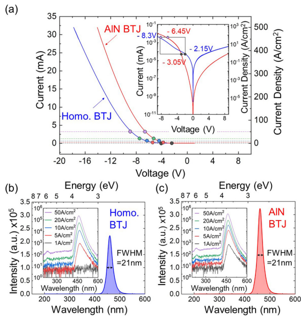
FIG. 3. (a) Current-voltage (I-V) characteristics (left axis) and J-V characteristics (right axis) for the two devices up to 500 A/cm 2 . The inset shows a log scale I-V curve, indicating a negative voltage turn-on, and the box indicates the region in which electroluminescence was collected. Electroluminescence spectra in the linear scale for (b) the homojunction and (c) the AlN BTJ LED at an injection current density of 50 A/cm 2 . Insets show EL spectra on a log scale at various injection current densities. The color of the dots in the IV-curve corresponds to the current density in the inset figures of the EL measurements. Both devices show peak emission at 460 nm, but the AlN BTJ LED has much higher emission at low current densities.
