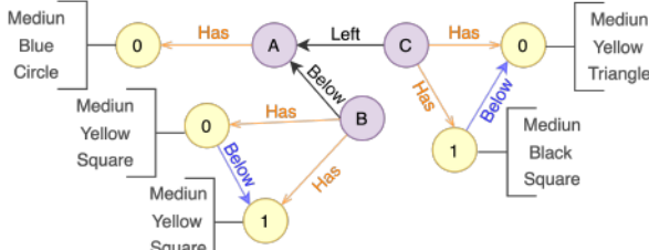
Figure 7: Scene-graph
