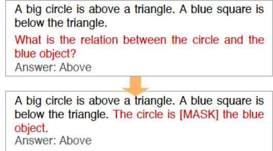
Figure 5: Convert a triplet of (paragraph, question, answer) into a single piece of text for the MLM task.
