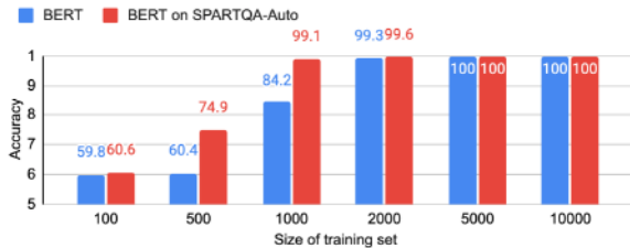
Figure 6: Learning curve of BERT and BERT further pretrained on SPARTQA-AUTO on bAbI.
