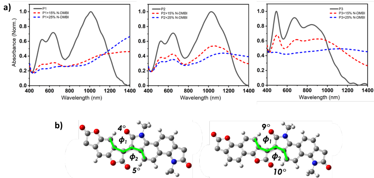
Figure 3(a) UV-Vis-NIR absorption spectra of the pristine and doped (at 15 and 25 mol% N-DMBI doping ratio) thin films of P1, P2, and P3. (b) DFT-optimized molecular model of the phenyl-bis-lactone and naphthalene-bis-lactone fragments ( \omega B97XD/6-31G**).
