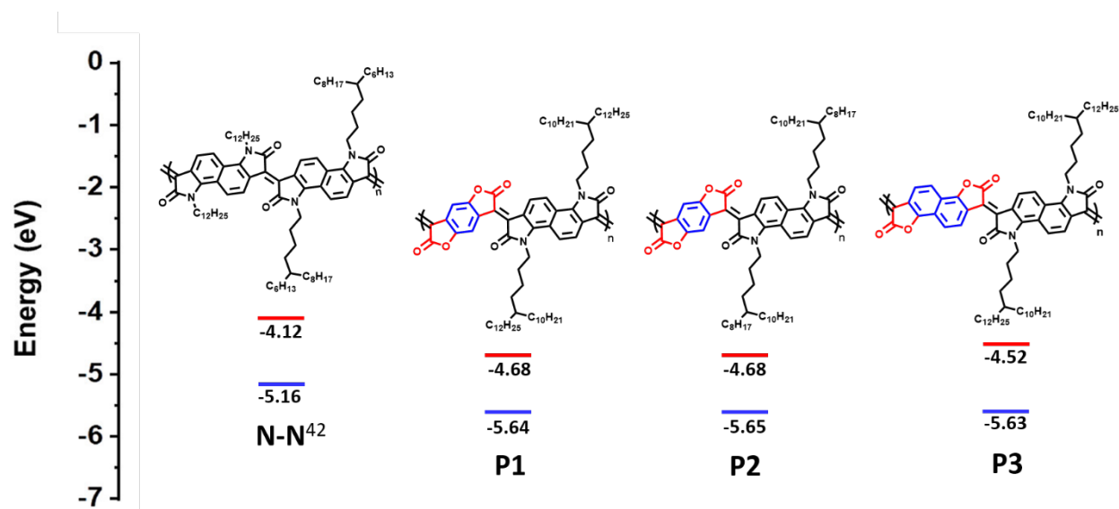
Figure 1. Chemical structures and calculated HOMO/LUMO of previous studied polymer (N-N) and new polymers, illustrating the effect of introducing bis-lactone units. HOMO is measured by photoelectron spectroscopy in air (PESA). LUMO is calculated from E_{\text{opt, gap}} and IP.
