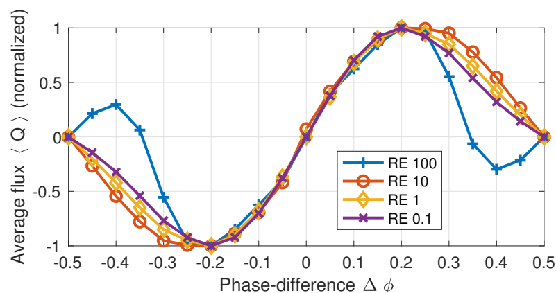
Figure 3. The effect of inter-paddle phase-difference on average flux at Reynolds number ( RE ) = 0.1, 1, 10, and 100 for four paddles with prescribed motion. Each flux is normalized by the maximum flux for that Reynolds number.
