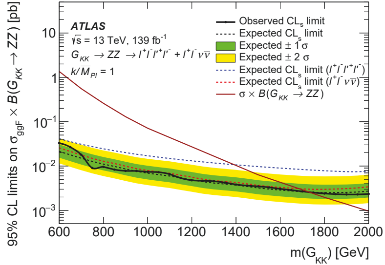
Figure 8: The upper limits at 95% CL on cross section times branching ratio \sigma \times B(G_{KK} \rightarrow ZZ) for a KK graviton produced with k/M_{Pl} = 1 . The black line indicates the observed limit. The green and yellow bands give the \pm 1\sigma and \pm 2\sigma uncertainties in the expected limits. The predicted production cross section times branching ratio as a function of the G_{KK} mass m(G_{KK}) is shown by the red solid line.
