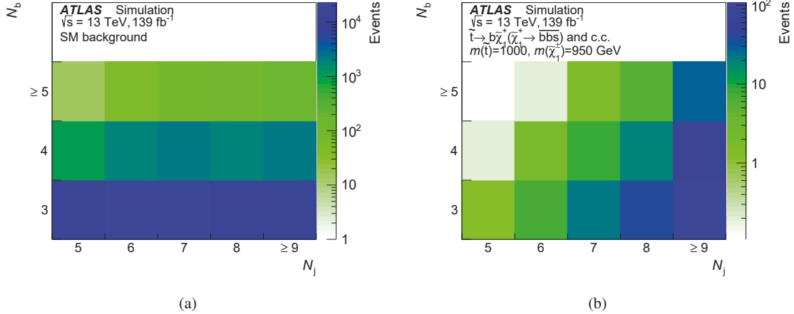
Figure 2: Predicted numbers of events as a function of jet multiplicity, N_j , and b -tagged jet multiplicity, N_b , for (a) SM background (multijet and top-quark production) and (b) top-squark pair production in the \tilde{t} \rightarrow \bar{b} \tilde{\chi}_1^+ (\tilde{\chi}_1^+ \rightarrow \bar{b} b s) (and c.c.) channel, for m_{\tilde{t}} = 1000 GeV and m_{\tilde{\chi}_1^\pm} = 950 GeV.
