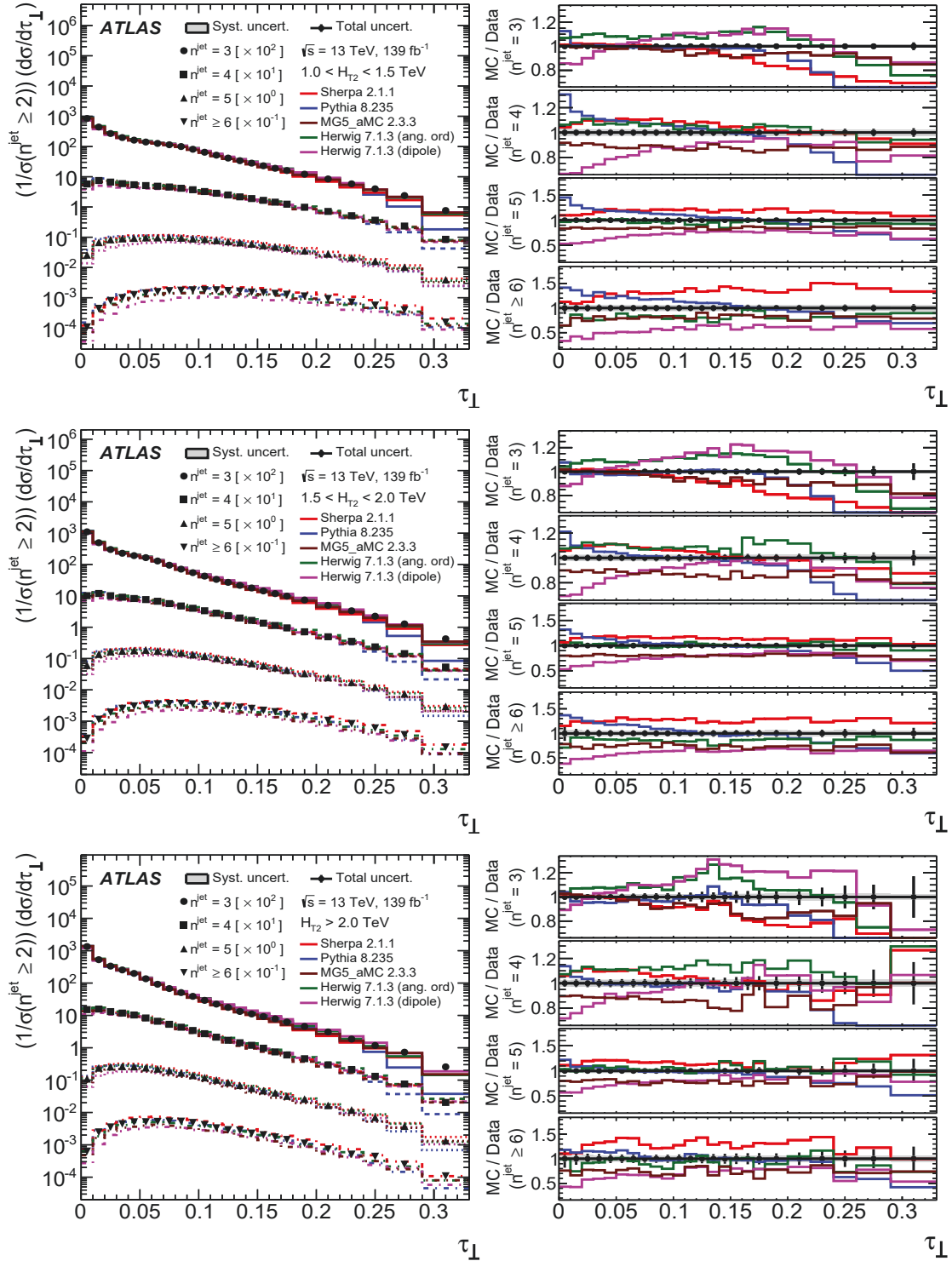
Figure 5: Comparison between data and MC simulation as a function of the transverse thrust \tau_\perp (see Eq. 1) for different jet multiplicities and energy scales. For illustration purposes, the corresponding differential cross section for each jet multiplicity is multiplied by 10^2 ( n^{\text{jet}} = 3 ), 10^1 ( n^{\text{jet}} = 4 ), 10^0 ( n^{\text{jet}} = 5 ), 10^{-1} ( n^{\text{jet}} \geq 6 ). The right panels show the ratios between the MC and the data distributions. The error bars show the total uncertainty (statistical and systematic added in quadrature) and the grey bands in the right panels show the systematic uncertainty.
