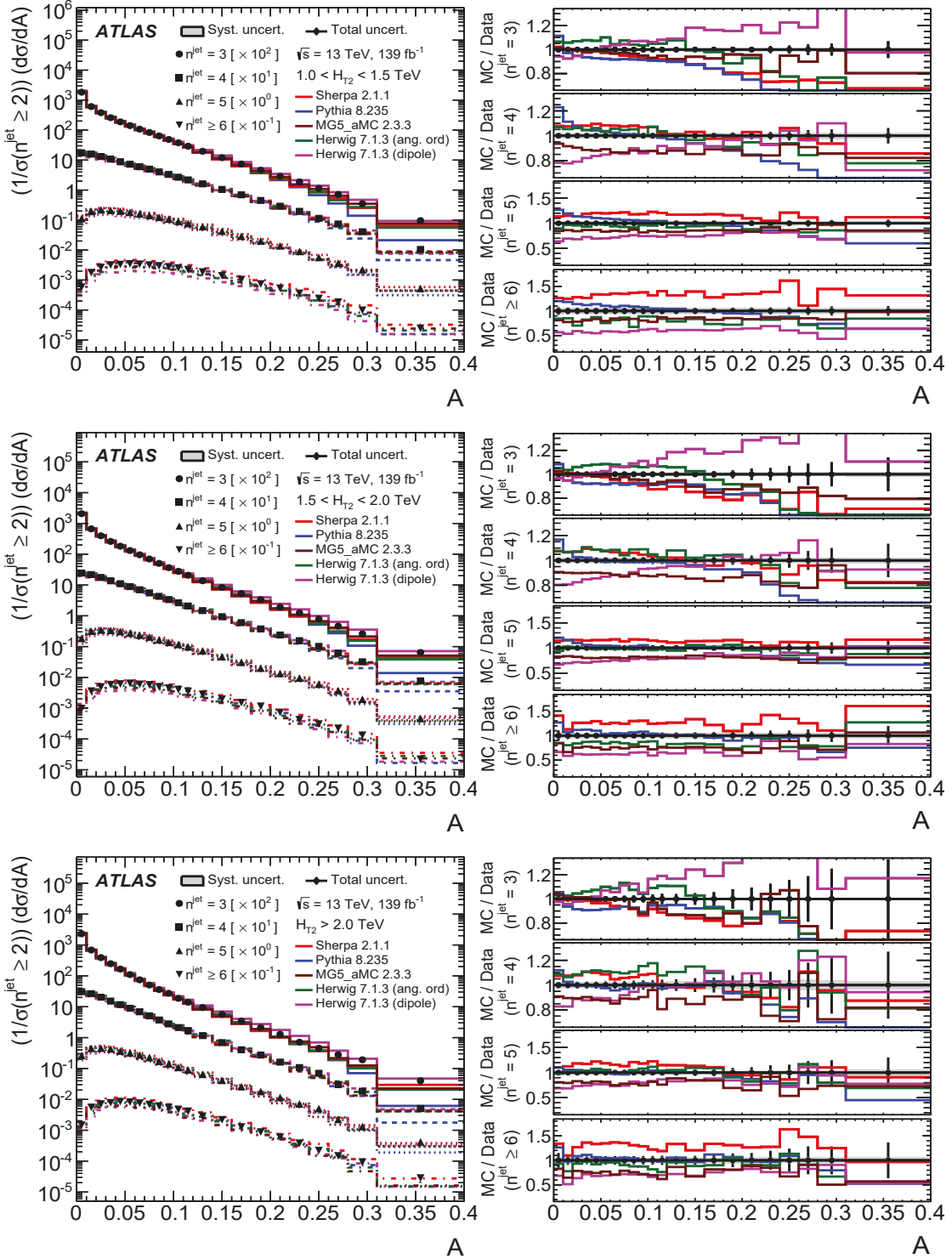
Figure 8: Comparison between data and MC predictions as a function of the aplanarity A (see Eq. 3) for different jet multiplicities and energy scales. For illustration purposes, the corresponding differential cross section for each jet multiplicity is multiplied by 10^2 ( n^{\text{jet}} = 3 ), 10^1 ( n^{\text{jet}} = 4 ), 10^0 ( n^{\text{jet}} = 5 ), 10^{-1} ( n^{\text{jet}} \geq 6 ). The right panels show the ratios between the MC and the data distributions. The error bars show the total uncertainty (statistical and systematic added in quadrature) and the grey bands in the right panels show the systematic uncertainty.
