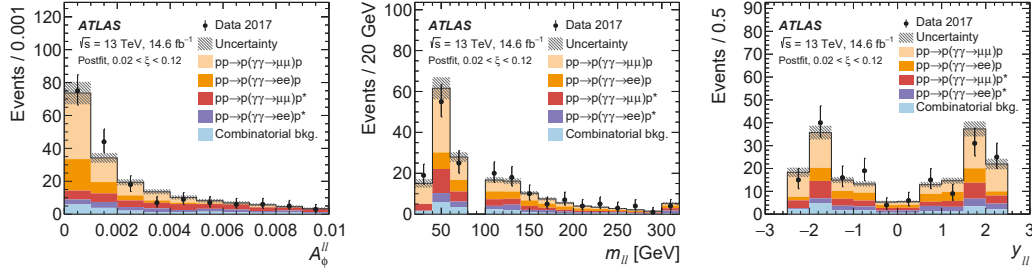
Figure 3: Distributions of dilepton acoplanarity A_{\phi}^{\ell\ell} (left), invariant mass m_{\ell\ell} (center), rapidity y_{\ell\ell} (right) satisfying \xi_{\ell\ell}, \xi_{\text{AFP}} \in [0.02, 0.12] , and |\xi_{\text{AFP}} - \xi_{\ell\ell}| < 0.005 for at least one AFP side. Events with 70 < m_{\ell\ell} < 105 GeV are vetoed. The total prediction comprises the signal and combinatorial background processes, where p^* denotes a dissociated proton. The simulated predictions are normalized to data to illustrate the expected signal composition. The rightmost bin of the m_{\ell\ell} distribution includes overflow. The hatched band indicates the combined statistical and systematic uncertainties of the prediction. Error bars denote statistical uncertainties of the data.
