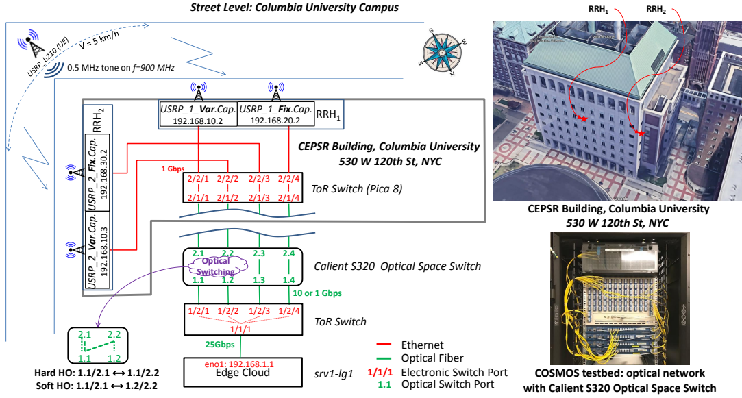
Fig. 3. Experimental setup: Two RRHs on each side of the CEPSR Building at Columbia University, with each composed of 2 USRPs. One USRP has a dedicated channel with fixed capacity through an optical link, another USRP has dynamic channel allocated by an SDN controller via OSS optical switching when wireless HO is underway. The UE moves around the building corner, passing from one RRH to another, invoking HO.
